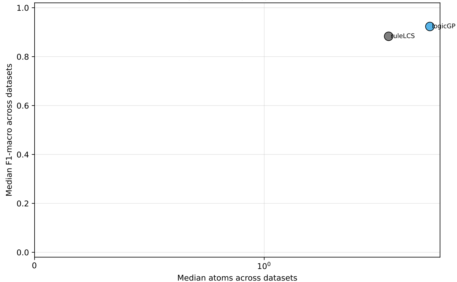
Executive Summary: median quality vs median model size
