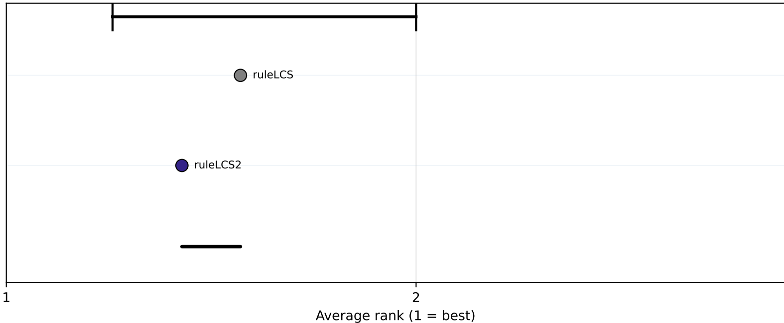
Critical Difference Diagram (F1 ranks across 7 datasets)
