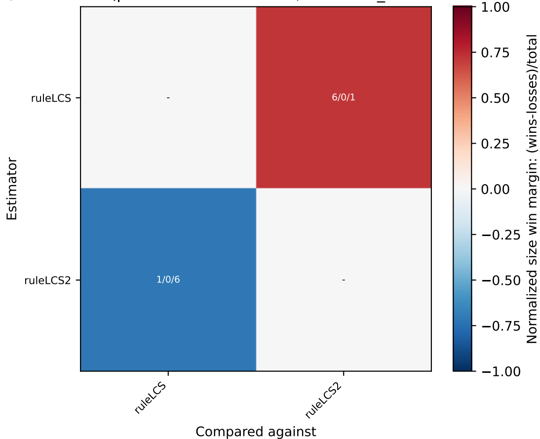
Win/Tie/Loss Matrix (pairwise over datasets, metric: n_atoms lower is better)
