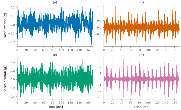
Figure 1. Raw drive-end acceleration signals at 0 HP, one 2048-sample window per class. (a) Normal, (b) inner race, (c) ball, (d) outer race. Each panel has its own y -axis scale: record RMS ranges from 0.066 g (Normal) to 0.425 g (outer race), so a shared scale would flatten three panels.
