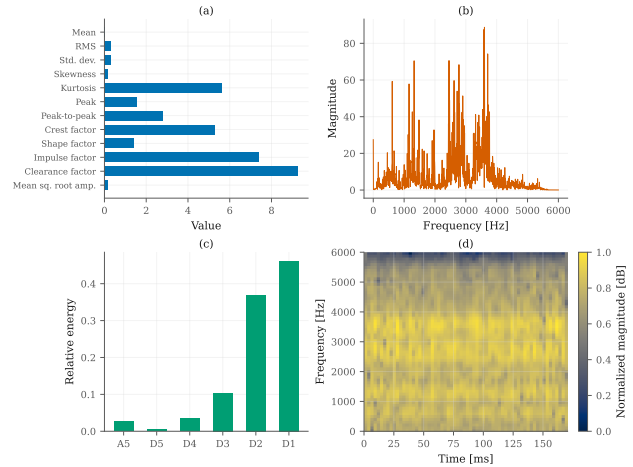
Figure 2. Same inner-race fault window at 0 HP under the four representations. (a) Time-domain statistics, (b) FFT magnitude, (c) db4 wavelet relative energy per band, (d) STFT spectrogram on the 64 \times 64 CNN grid, not the 16 \times 64 grid that enters the comparison. The twelve descriptors of (a) do not share units; wavelet bands run from coarsest approximation (A5) to finest detail (D1).
