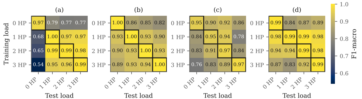
Figure 3. Macro-F1 for every (training load, test load) pair, averaged over the three vector classifiers and 5 folds. (a) Statistical, (b) FFT, (c) Wavelet db4, (d) STFT spectrogram. The diagonal is a reference cell, boxed for orientation, and takes part in neither Friedman nor the ANOVA: with a single Normal recording per load it does not admit a record-level split.
