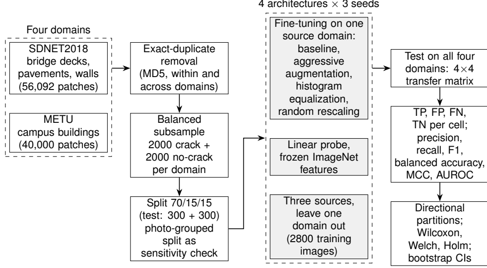
Fig. 1 Experimental pipeline. Four domains are deduplicated, subsampled to the same size and class balance, and split; each architecture is then trained under three regimes (fine-tuning on one source domain, as a baseline and with three training-time interventions; linear probe on frozen features; three-source training with one domain held out) and every model is tested on the test split of all four domains. TP, FP, FN and TN are true and false positives and negatives; MCC, Matthews correlation coefficient; AUROC, area under the receiver operating characteristic curve; CI, confidence interval
