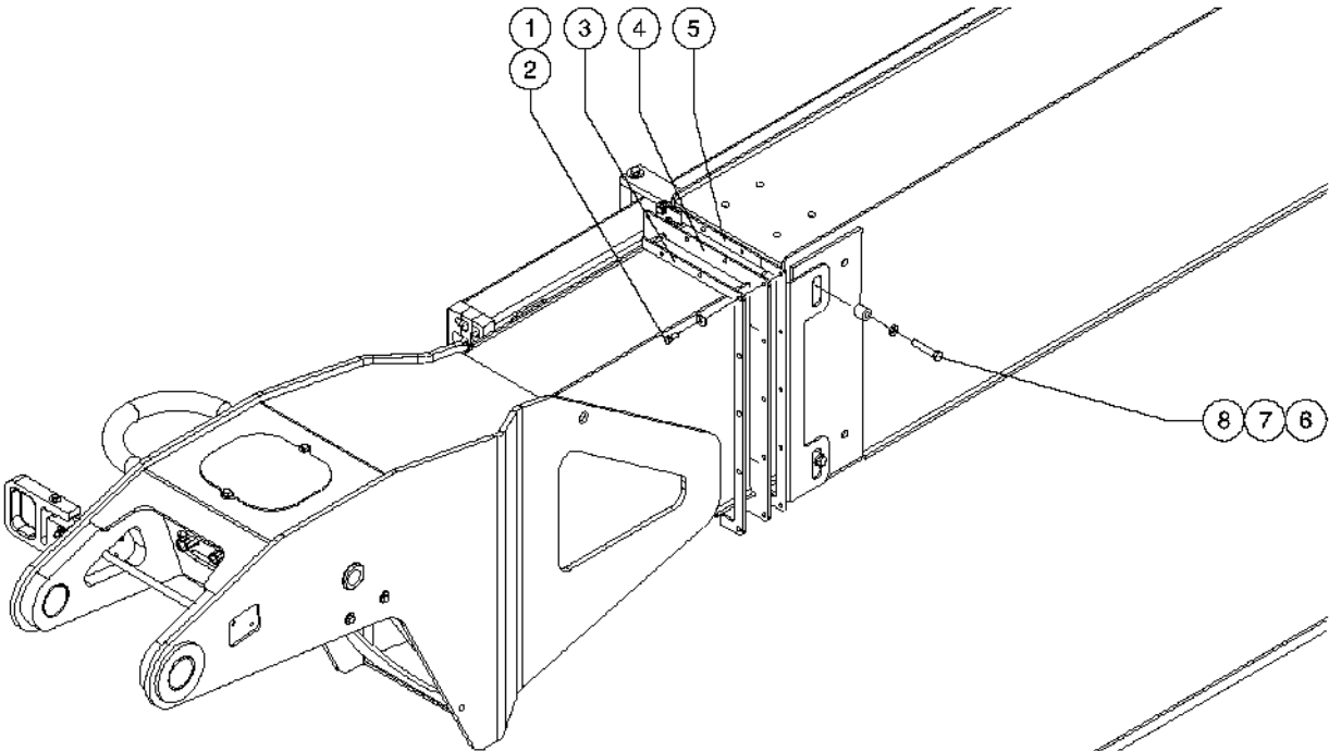
Primary Boom
