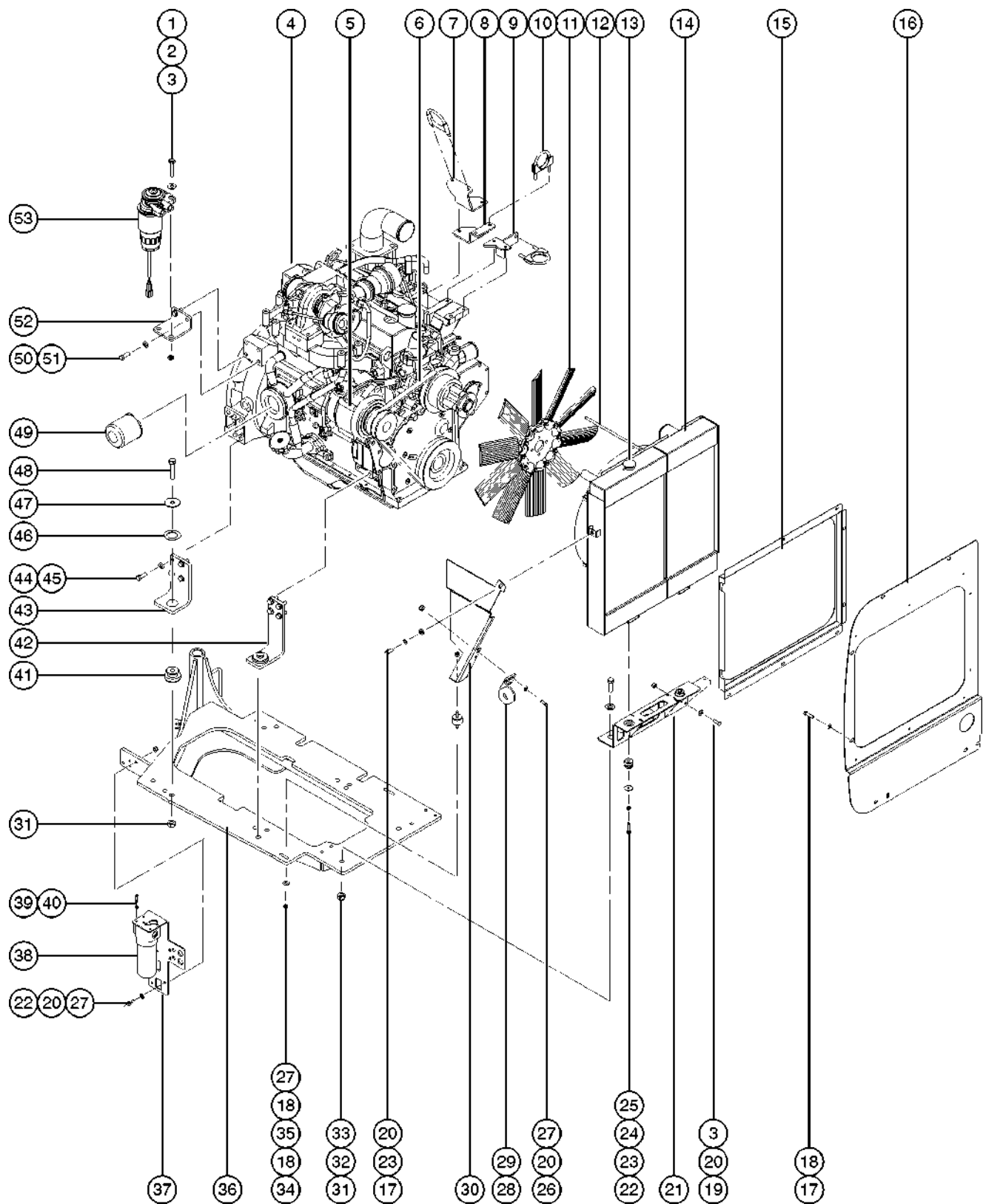
402.2 Cummins B3.3T Engine, View 2 (from SN 951)
