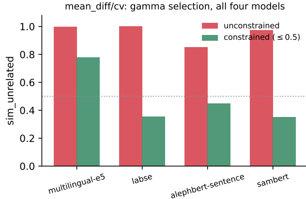
Figure 1: Same phenomenon, all four models, mean-difference direction, cross-validated selection: unconstrained selection lands on \text{sim\_unrelated} \geq 0.85 every time; the constrained version lands under 0.45 on three of four (multilingual-e5 is the exception discussed above).
