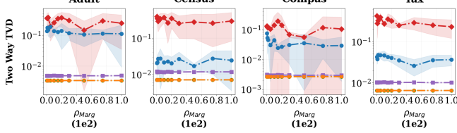
(b) Two-way TVD (log scaled) as a function of marginals \rho_{marg} .
