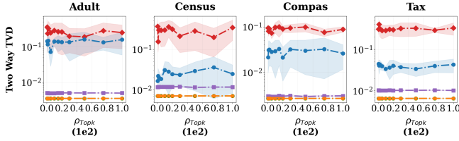
(a) Two-way TVD (log scaled) for each dataset as a function of \rho_{Topk} .
