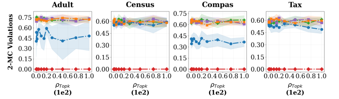
(a) 2-MCs violations for each dataset as a function of \rho_{Topk} .
