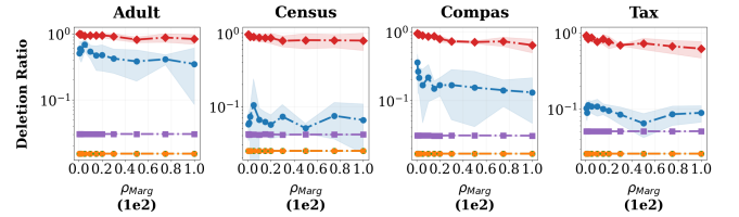
(b) Deletion ratio (log scaled) as a function of marginals \rho_{marg} .
