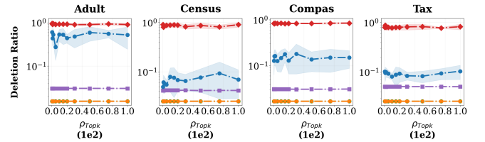
(a) Deletion ratio (log scaled) for each dataset as a function of \rho_{Topk} .
