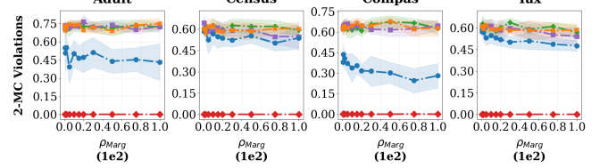
(b) 2-MCs violations as a function of marginals \rho_{marg} .
