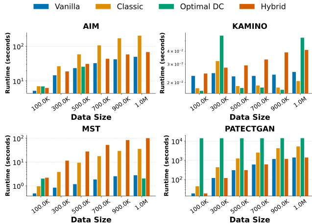
Figure 6: Runtime as a function of the synthetic data size for the Census dataset.
