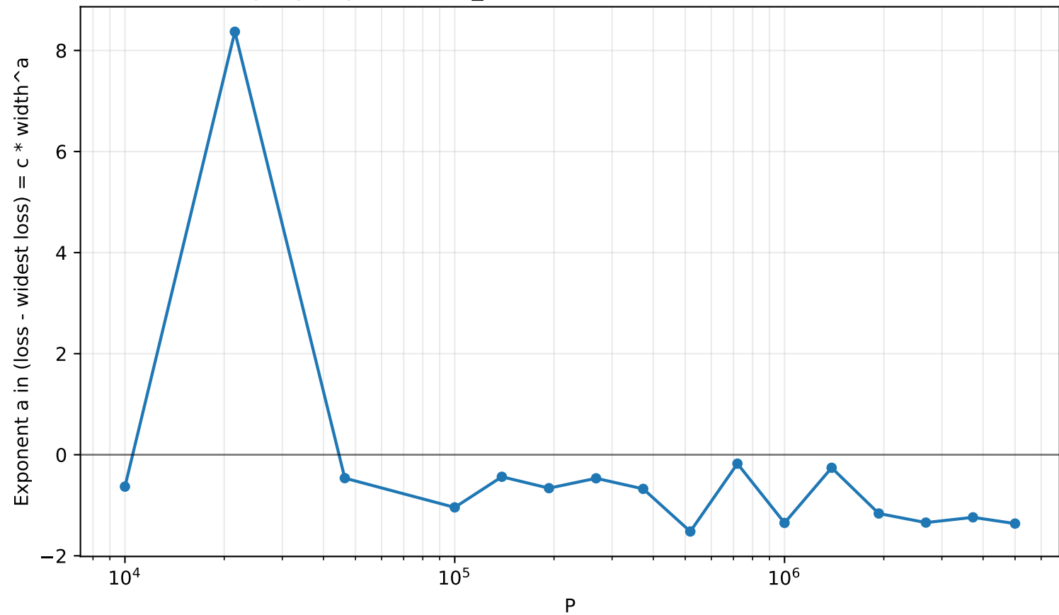
Log-log slope of (train_loss - widest-network loss)(width) vs P
