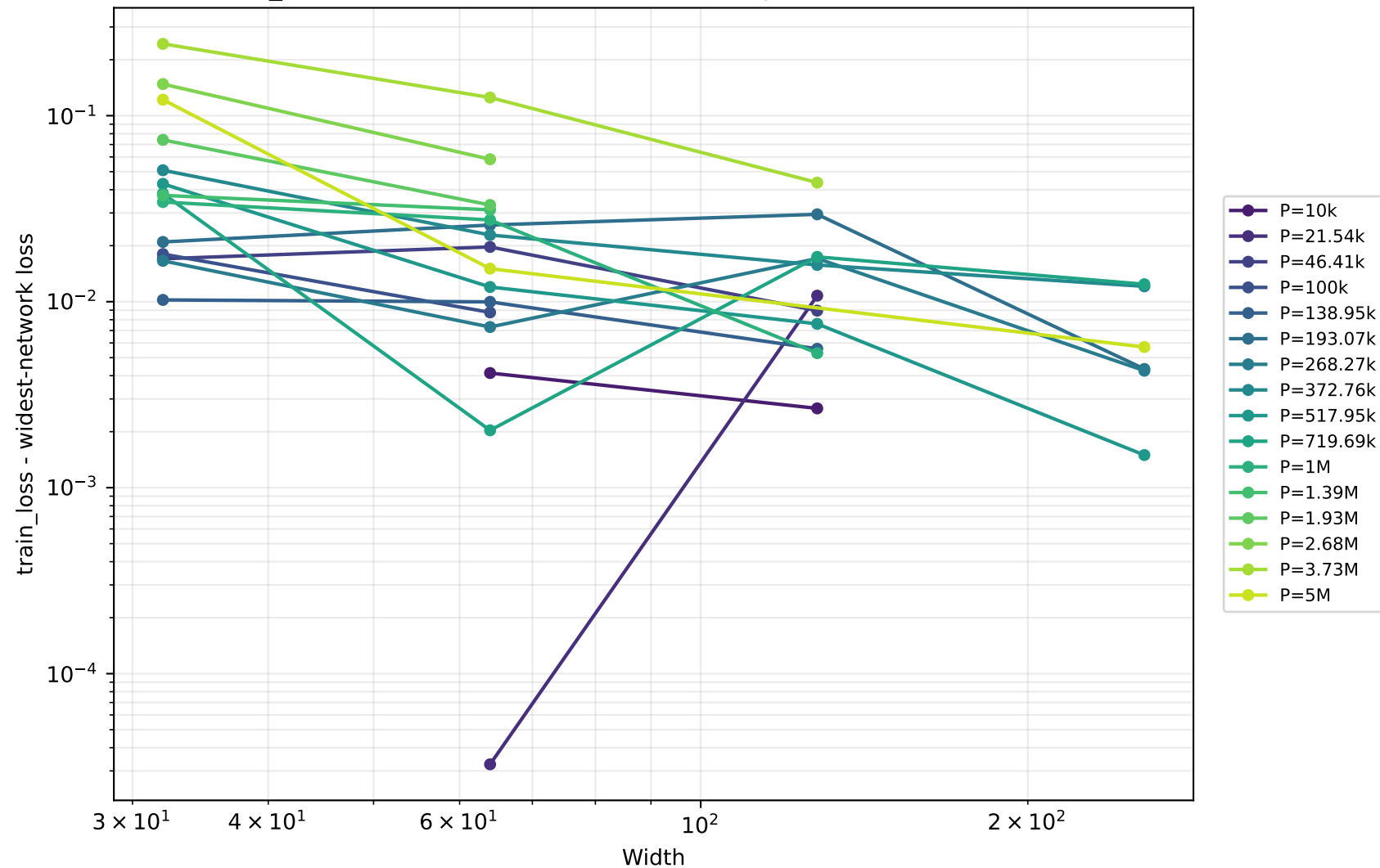
train_loss - widest-network loss vs width by P (available P selection)
