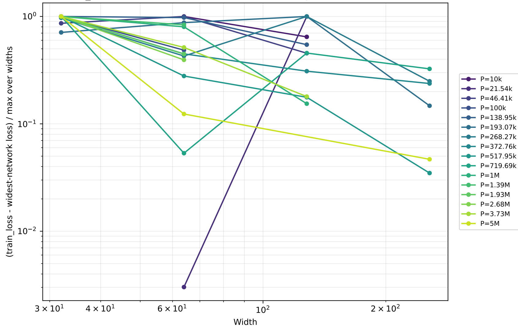
(train_loss - widest-network loss) / max vs width by P (available P selection)
