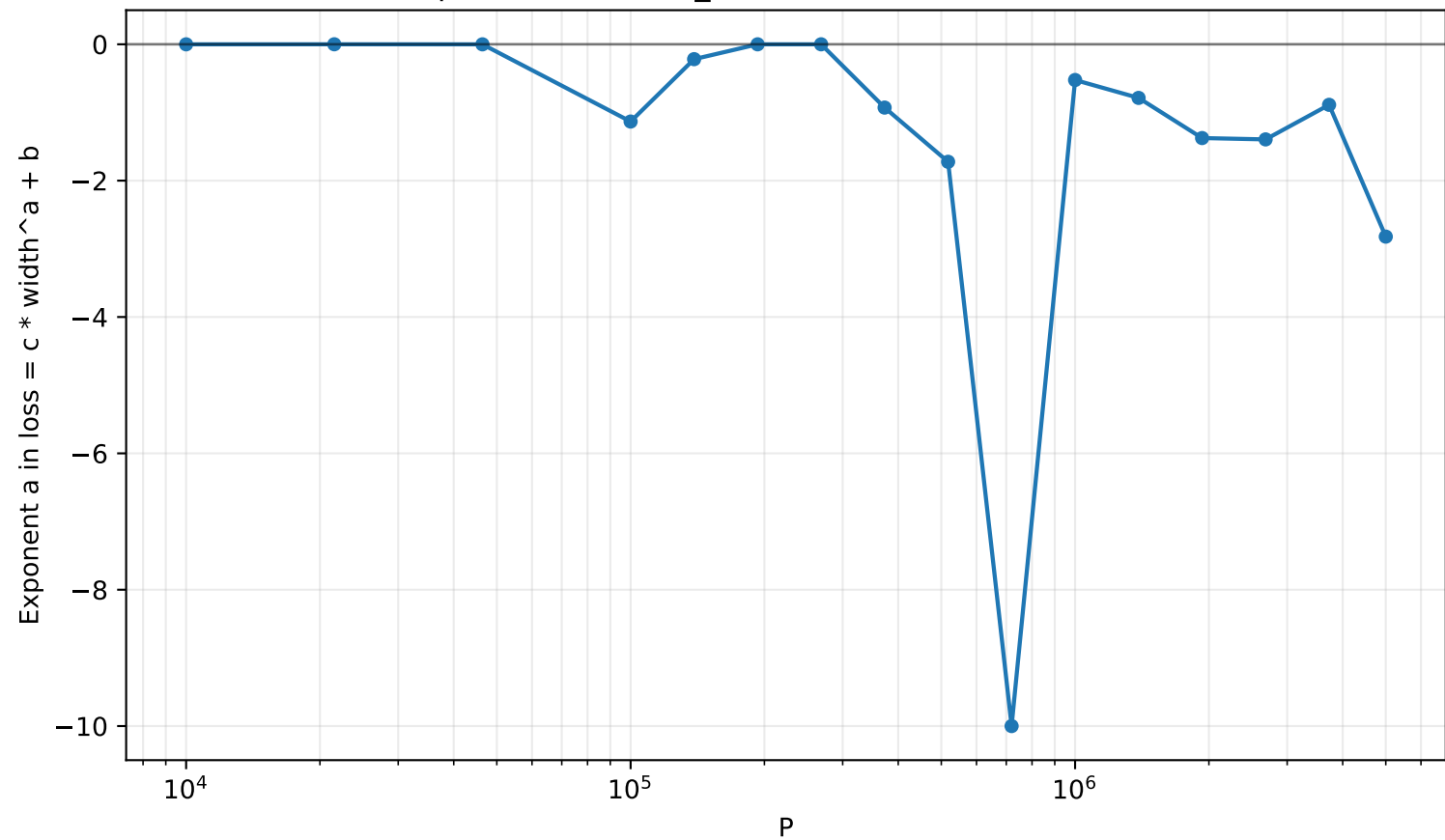
Exponent a in \text{train\_loss}(\text{width}) = c * \text{width}^a + b
