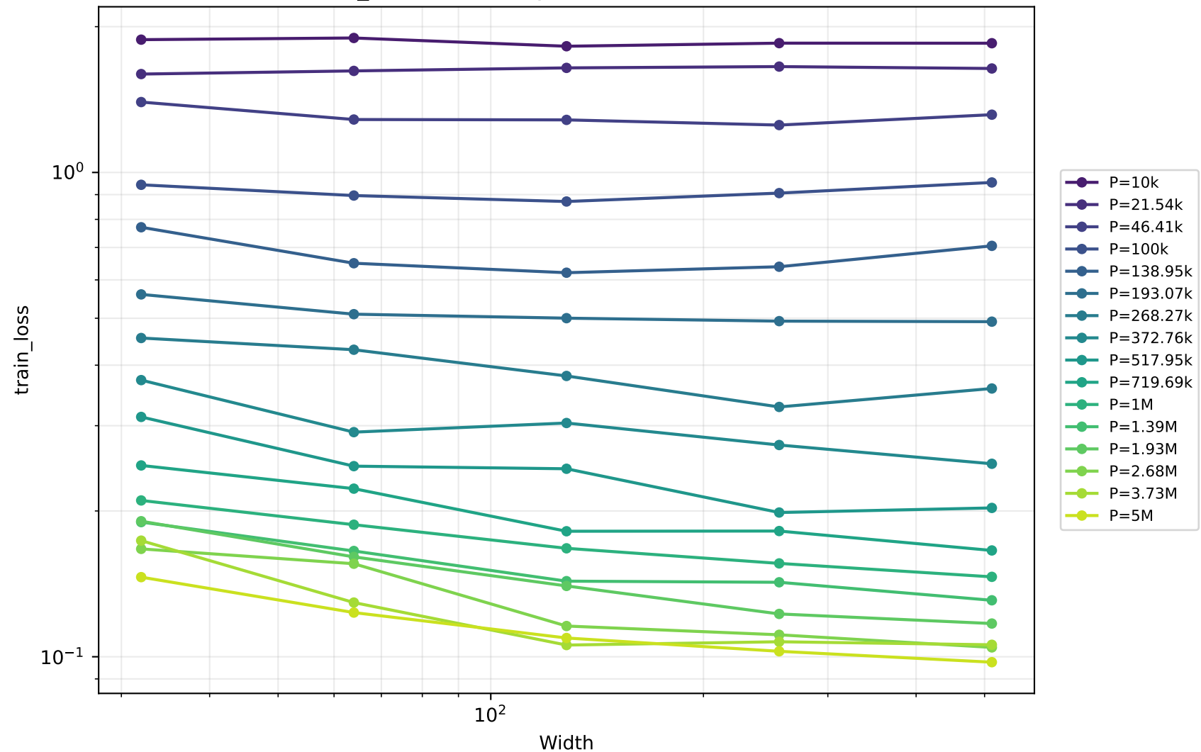
train_loss vs width by P (available P selection)
