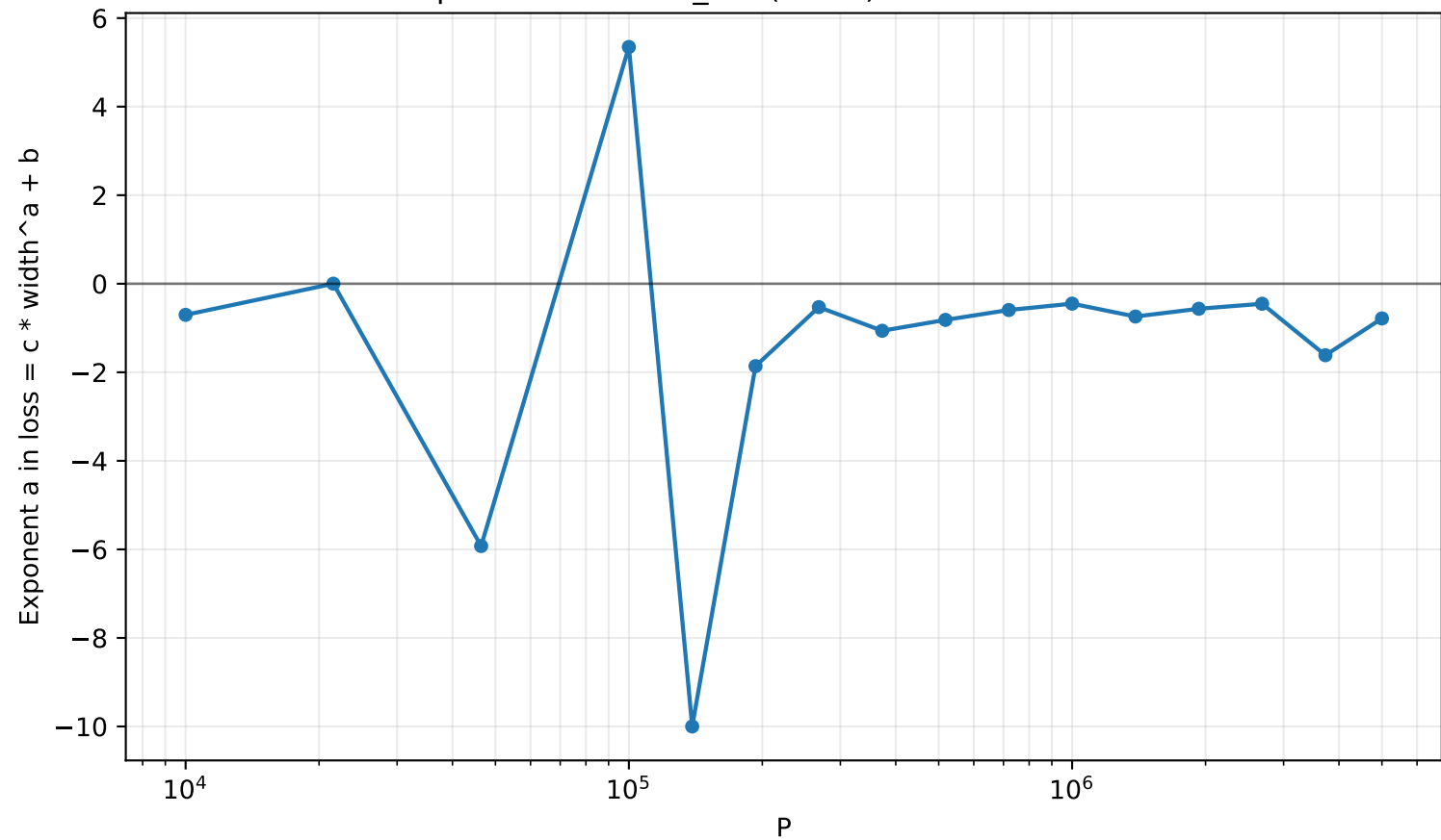
Exponent a in \text{train\_loss}(\text{width}) = c * \text{width}^a + b
