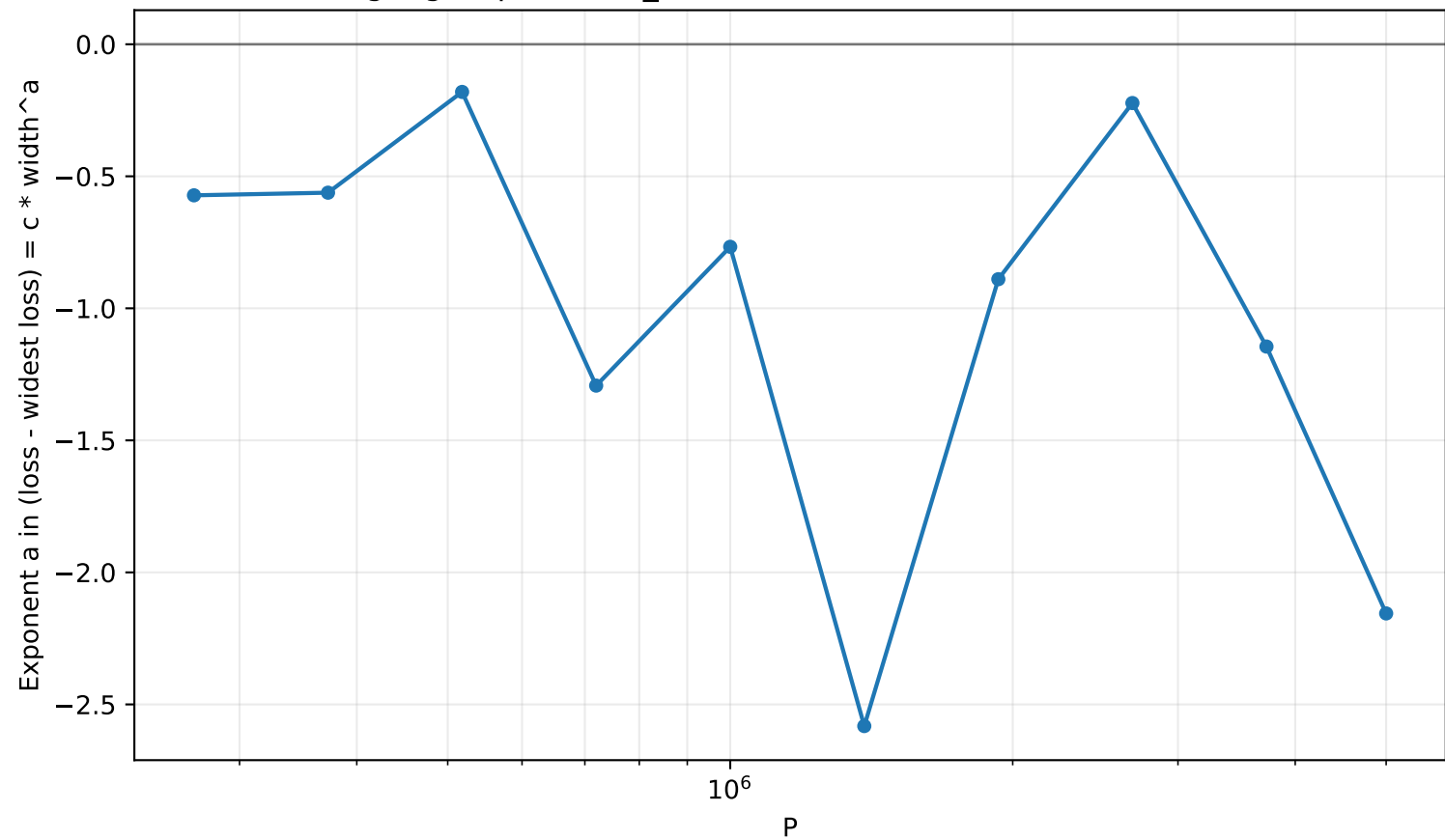
Log-log slope of (val_loss - widest-network loss)(width) vs P
