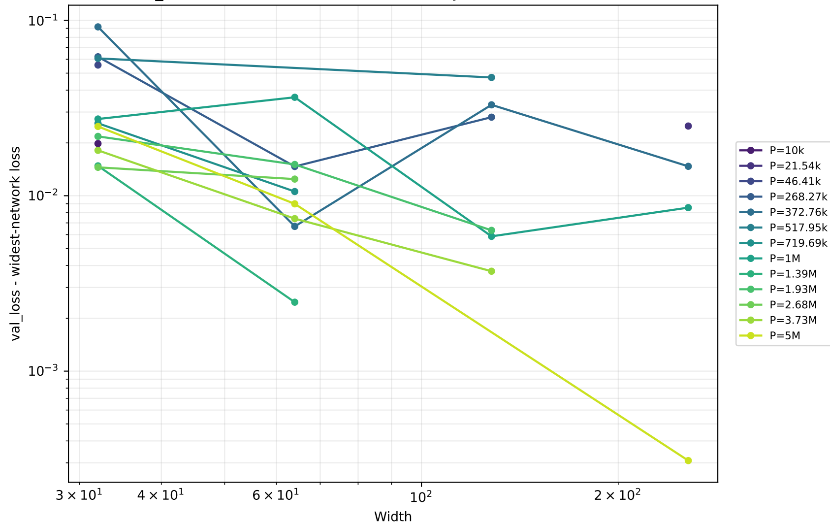
val_loss - widest-network loss vs width by P (available P selection)
