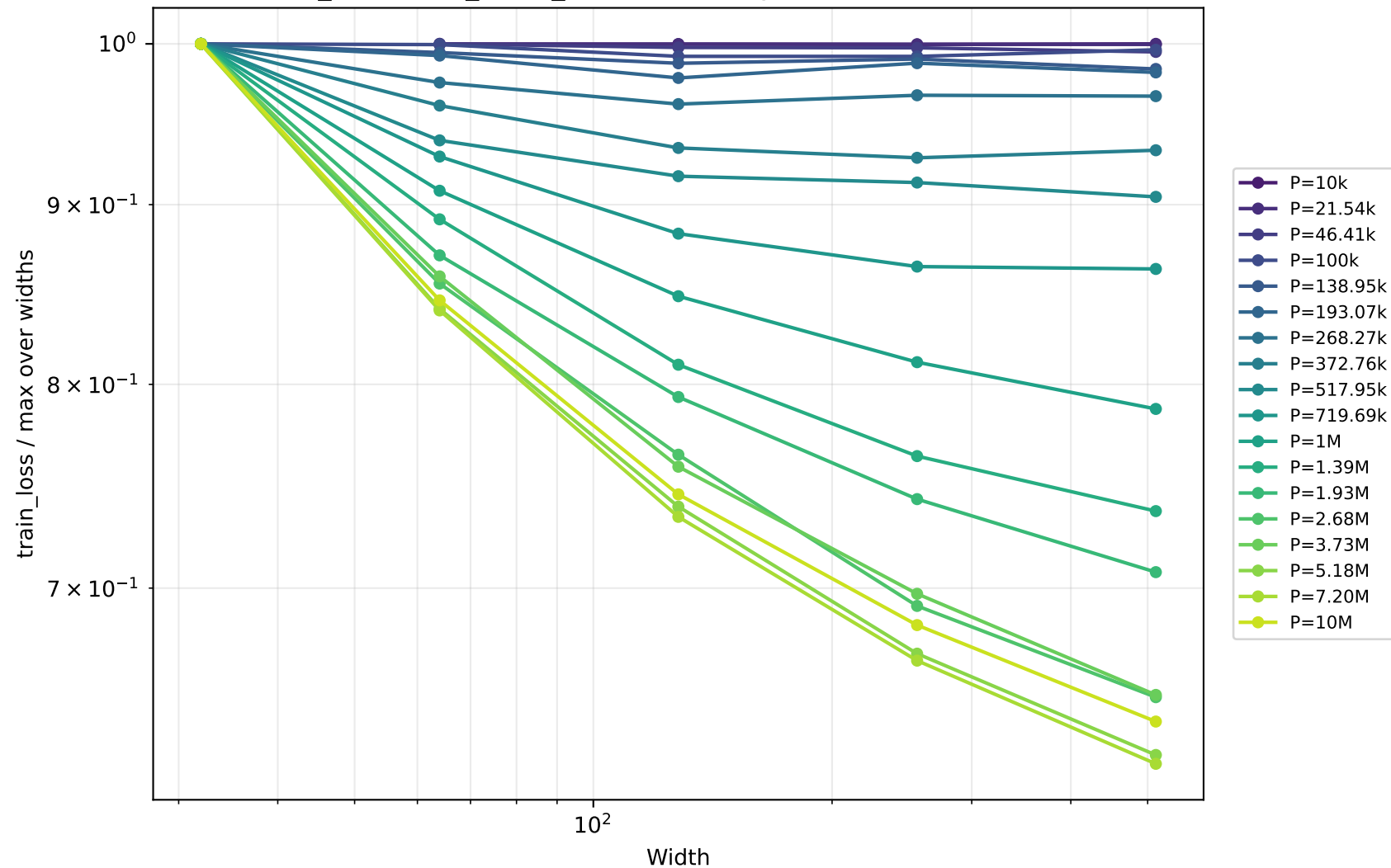
train_loss / max_width_loss vs width by P (available P selection)
