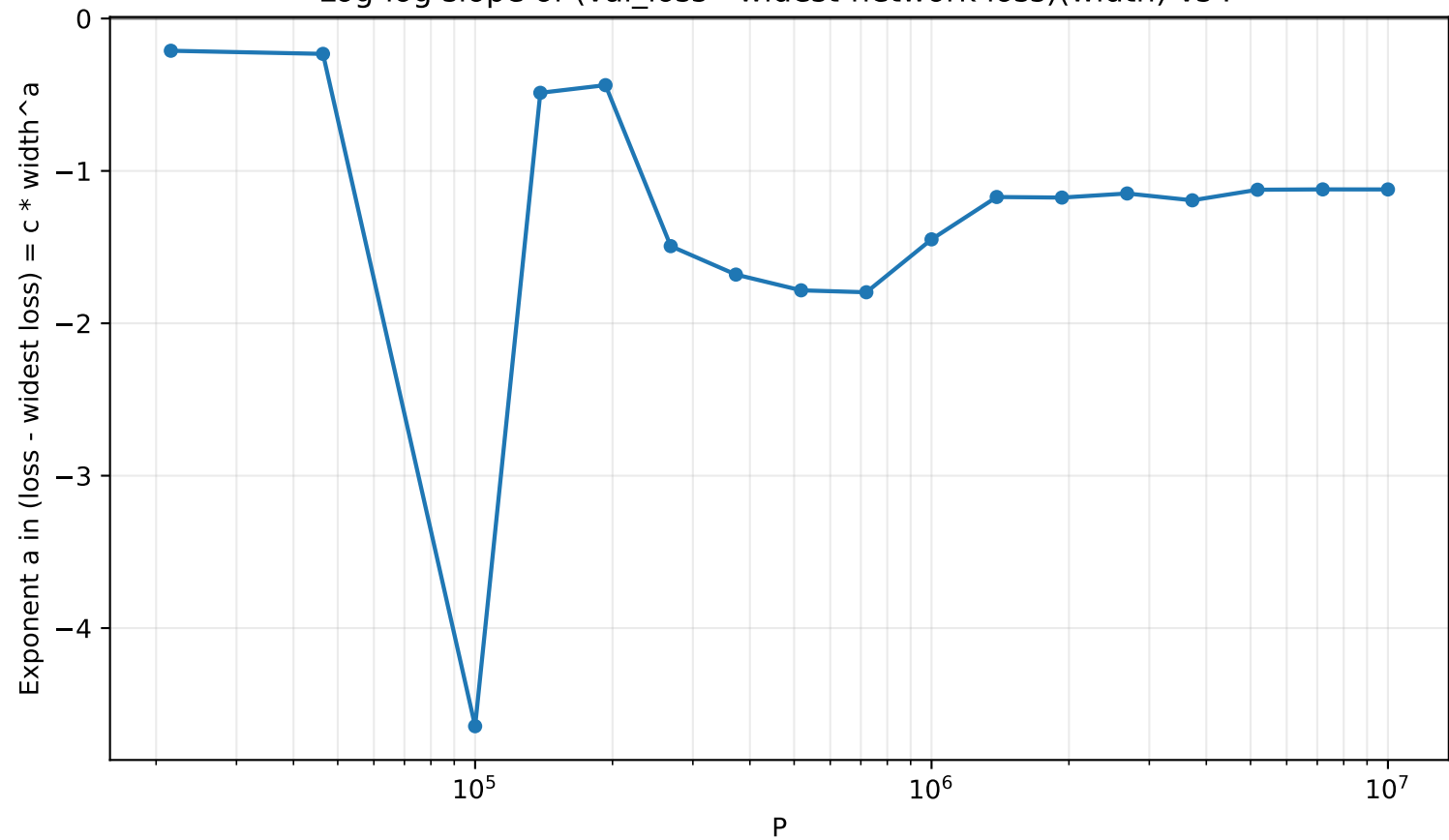
Log-log slope of (\text{val\_loss} - \text{widest-network loss})(\text{width}) vs P
