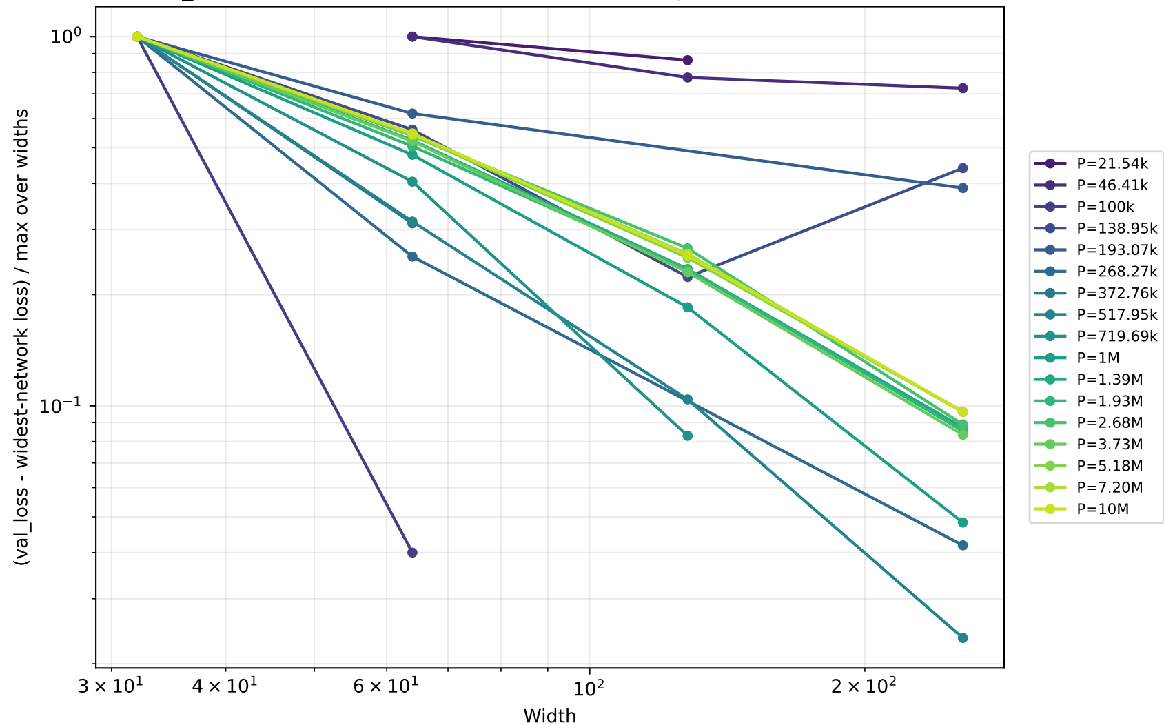
(val_loss - widest-network loss) / max vs width by P (available P selection)
