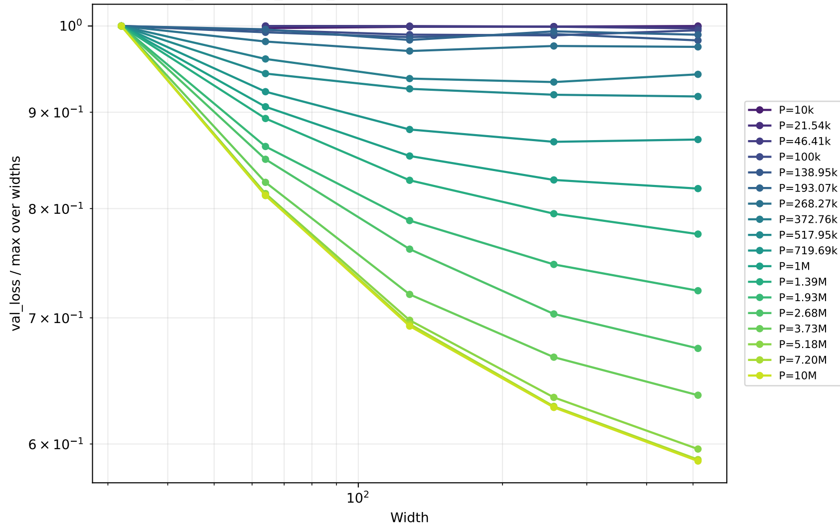
val_loss / max_width_loss vs width by P (available P selection)
