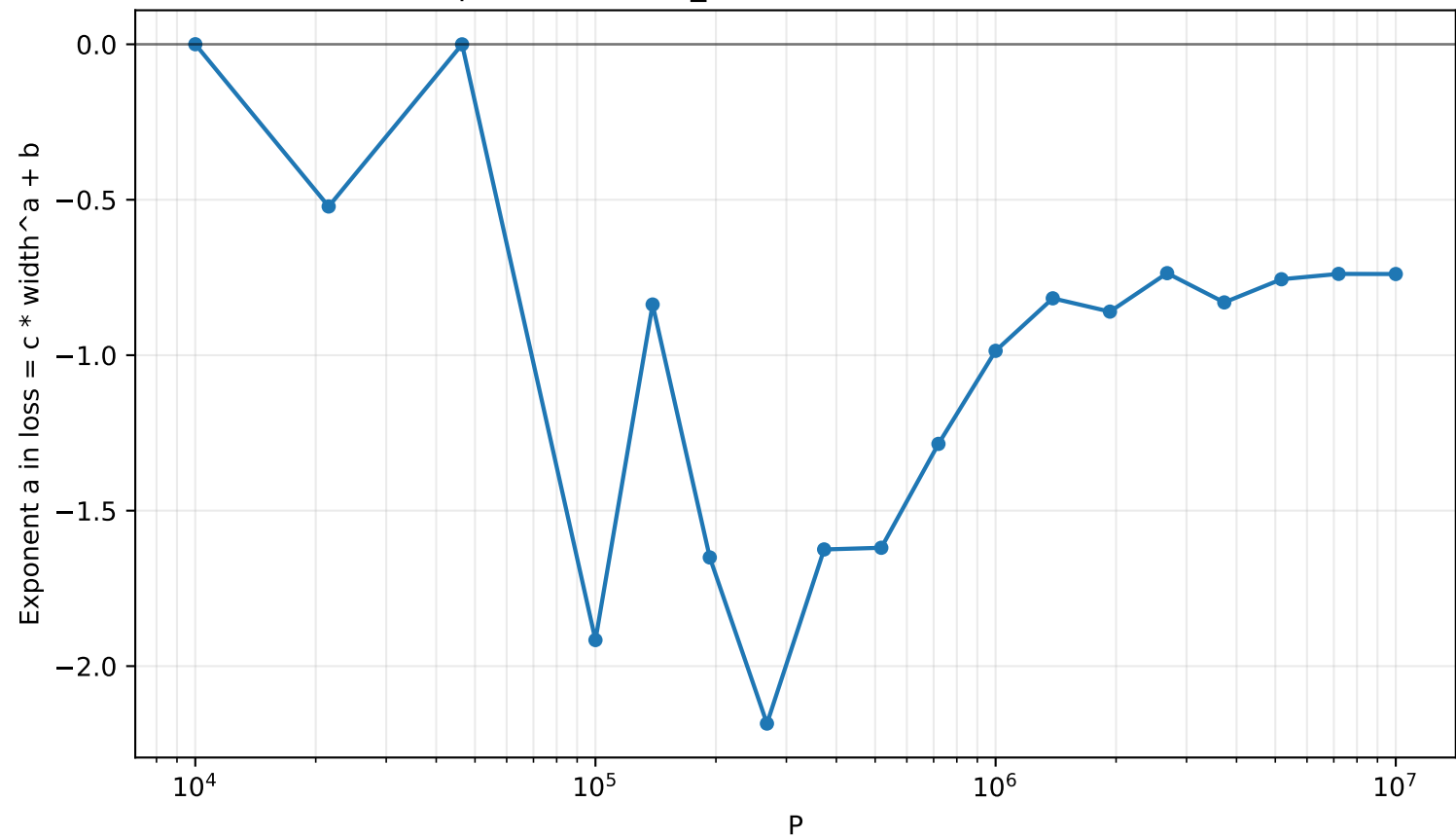
Exponent a in \text{val\_loss}(\text{width}) = c * \text{width}^a + b
