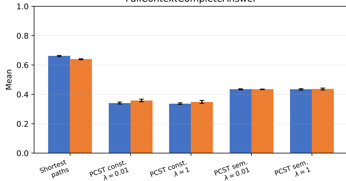
FullContextCompleteAnswer
