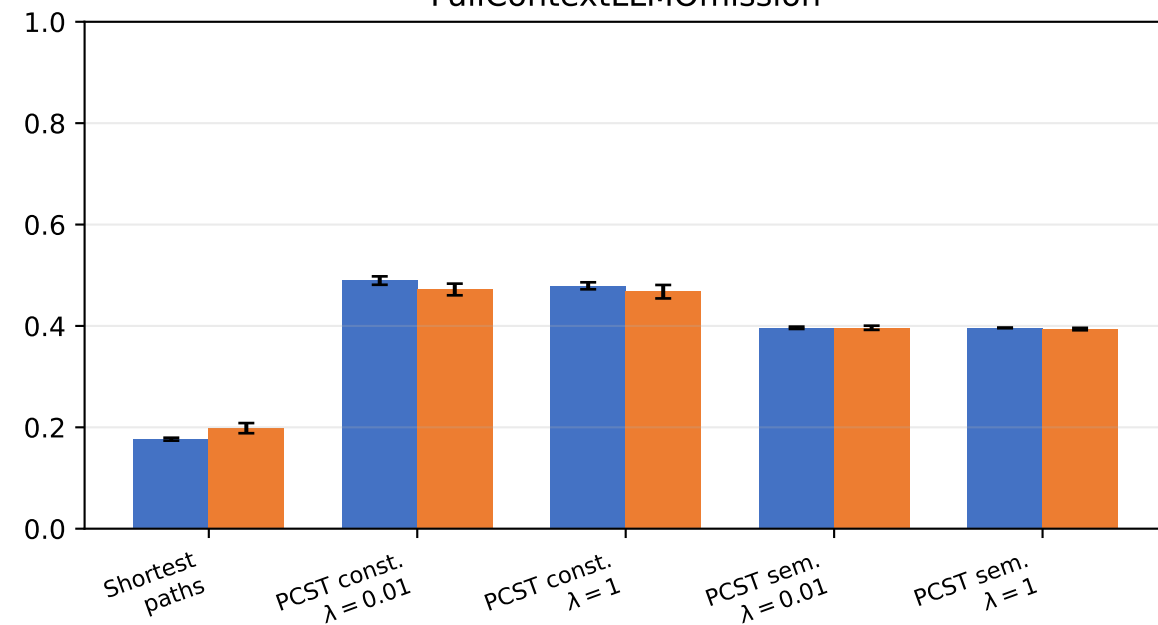
FullContextLLMOmission
