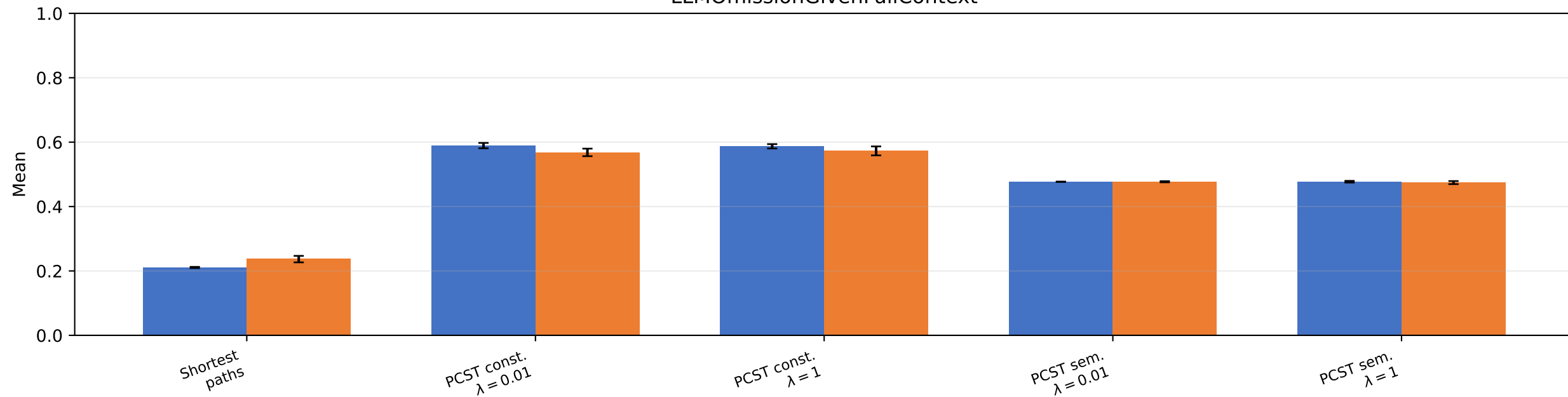
LLMOmissionGivenFullContext
