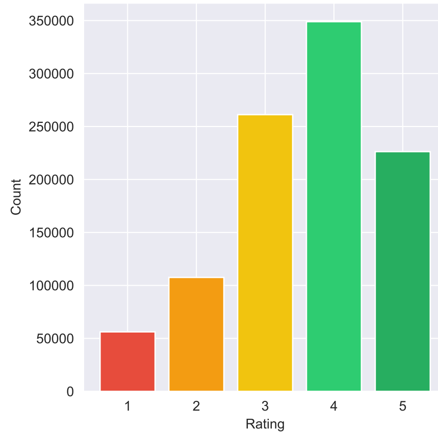
Rating Distribution
