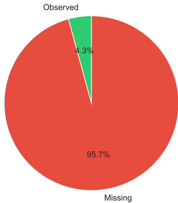
Matrix Sparsity
