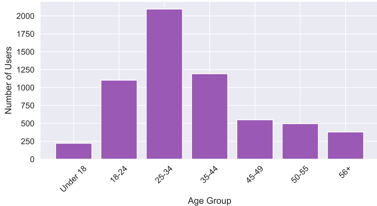
Age Distribution
