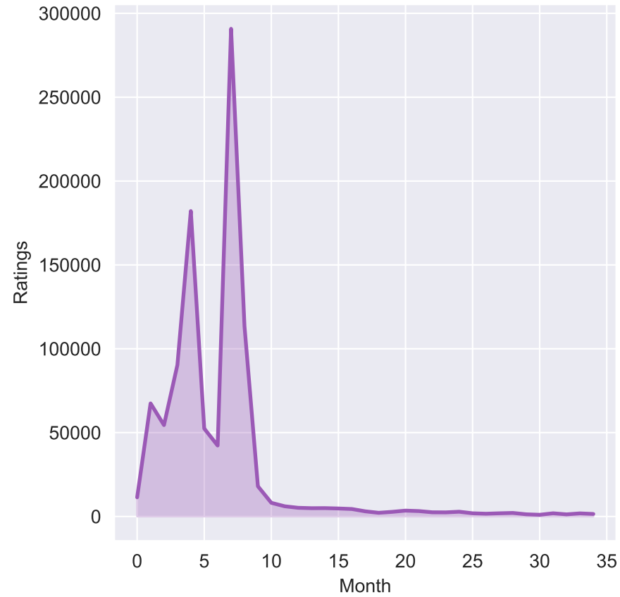
Temporal Volume
