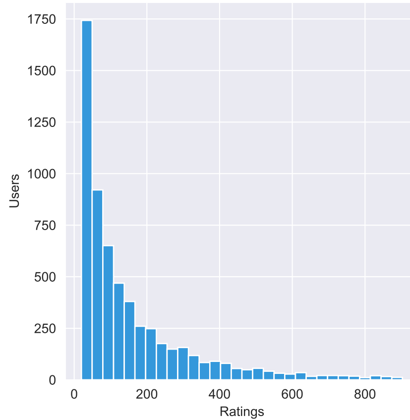
Rating Distribution
