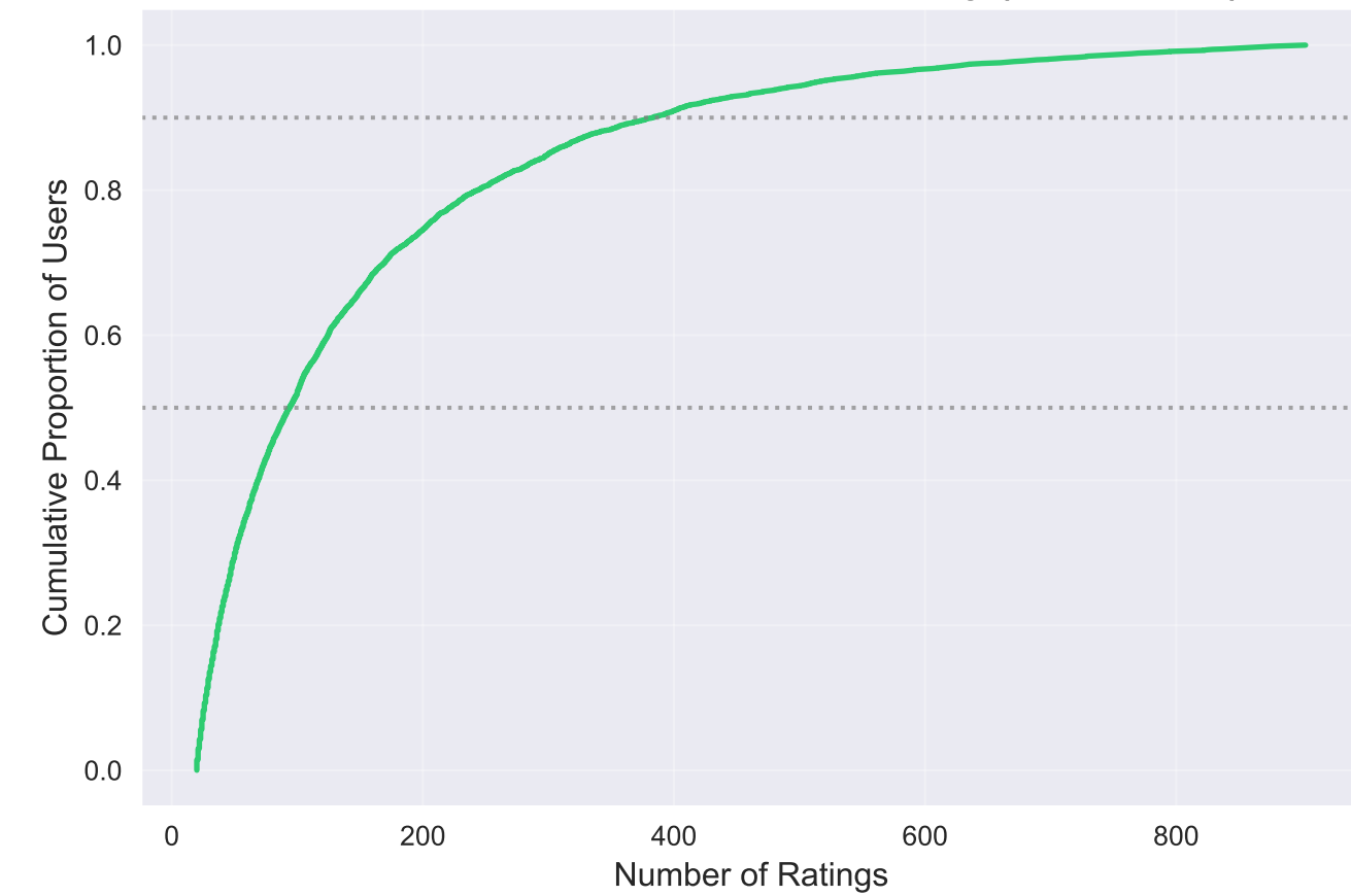
Cumulative Distribution of User Activity (bottom 99%)
