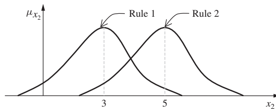
FIGURE 7.6 Input membership functions for x_2 .
