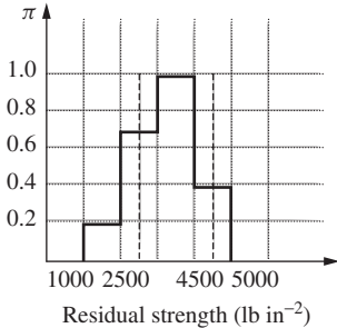
FIGURE 15.8 Possibility distribution for the residual strength of the bridge.
