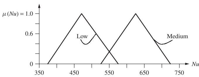
FIGURE P5.32c Output for Mamdani inference
