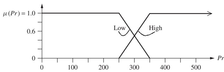
FIGURE P5.32b Input for Prandtl number
