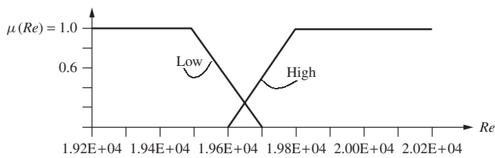
FIGURE P5.32a Input for Reynolds number
