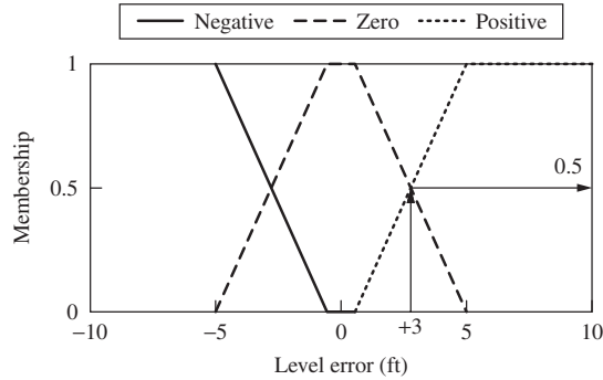
FIGURE 13.23 Resolution of input for Example 13.4.
