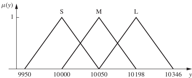
FIGURE 8.22 Partitioning for the output variable, y .
