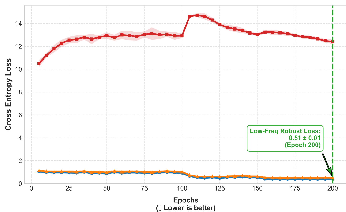
CIFAR-10 Test Loss vs. Epochs (5 Seeds Mean \pm SD)
