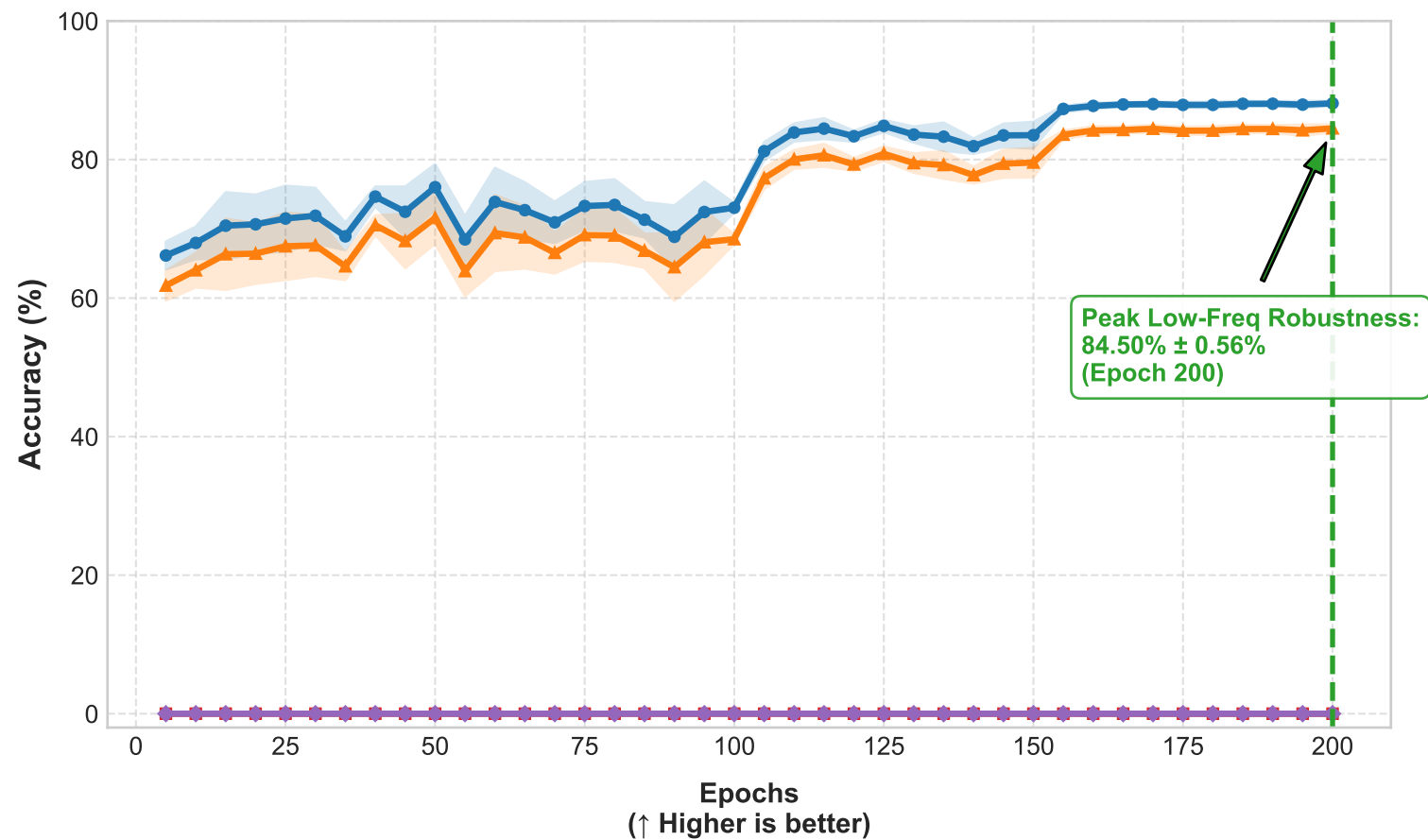
CIFAR-10 Test Accuracy vs. Epochs (5 Seeds Mean \pm SD)
