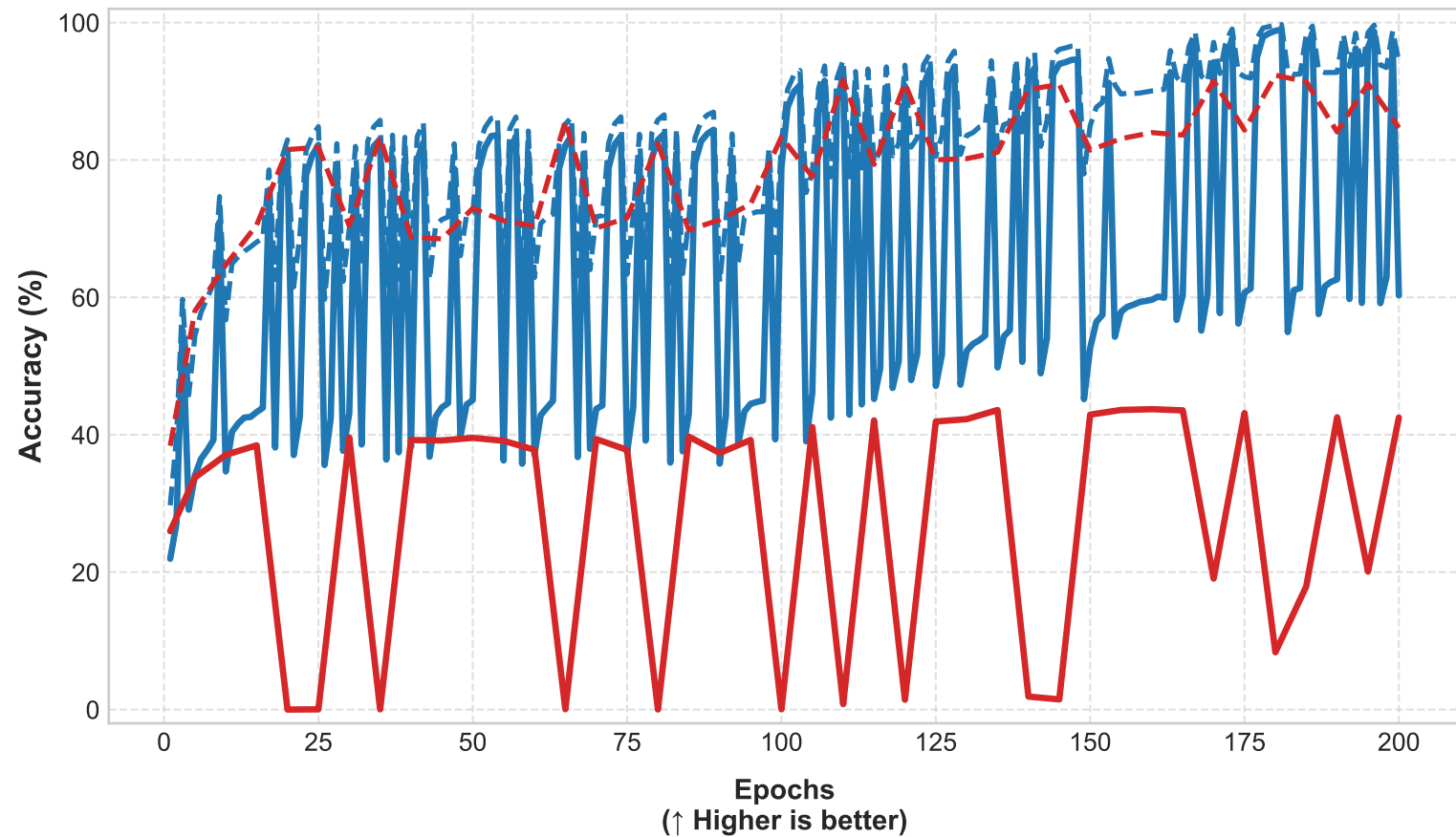
Training & Test Accuracy (TensorBoard Log)
