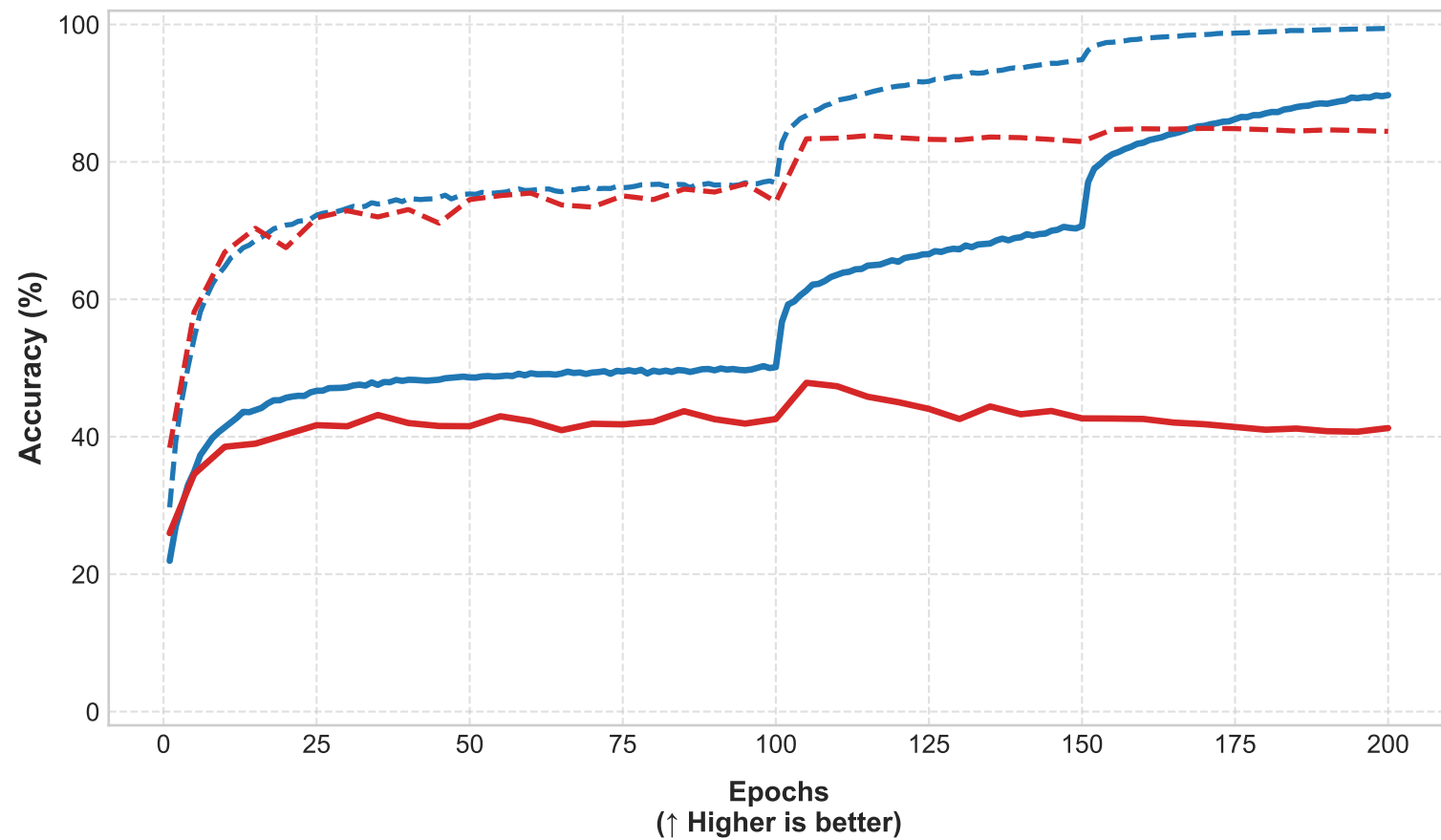
Training & Test Accuracy (TensorBoard Log)
