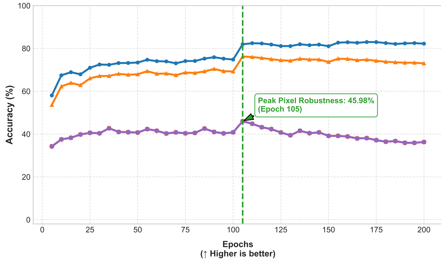
CIFAR-10 Test Accuracy vs. Epochs
