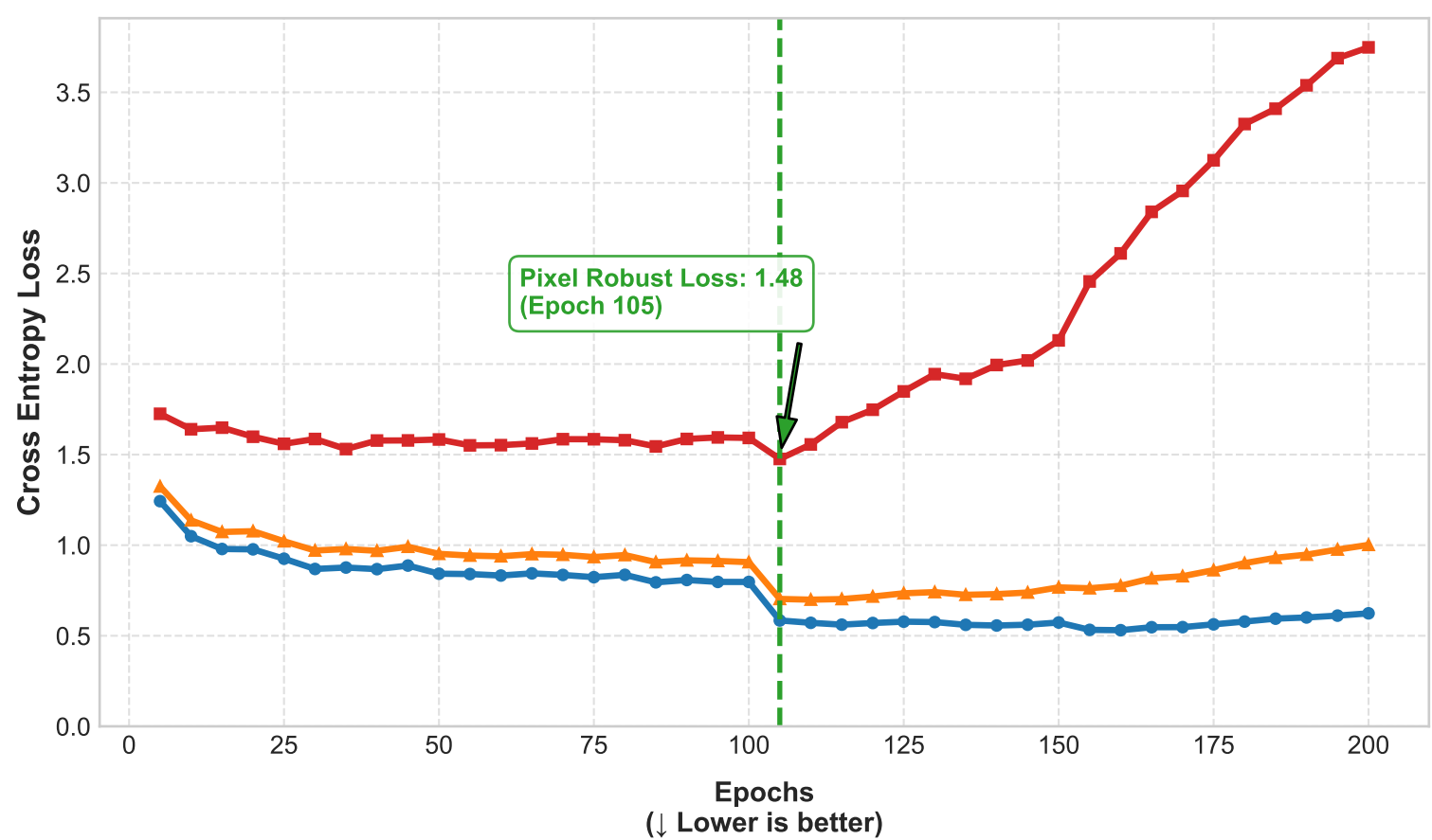
CIFAR-10 Test Loss vs. Epochs
