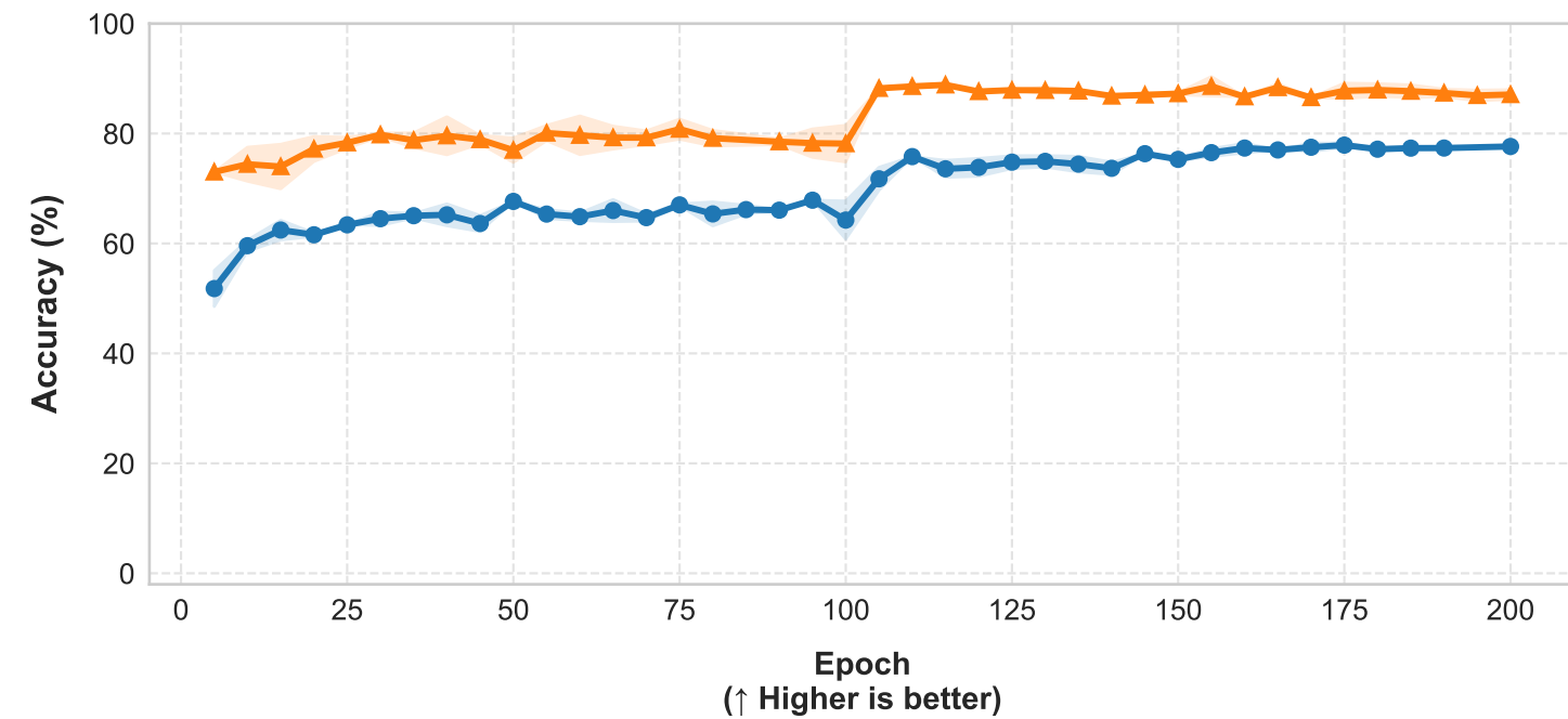
Low-Frequency-PGD-20 Test Accuracy
