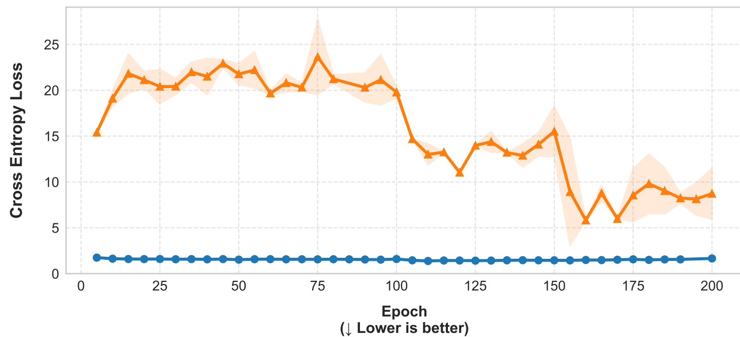
Pixel-PGD-20 Test Loss
