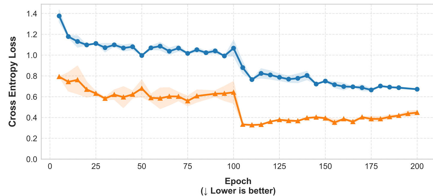
Low-Frequency-PGD-20 Test Loss
