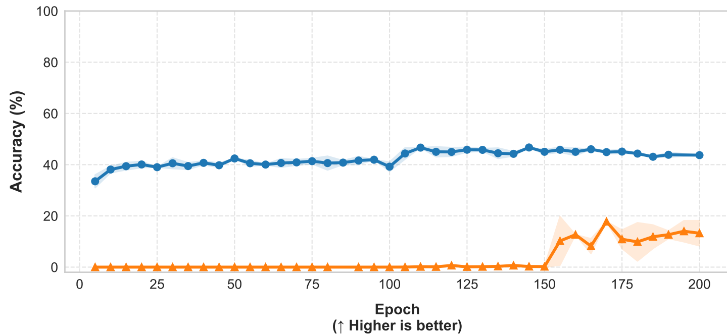
Pixel-PGD-20 Test Accuracy
