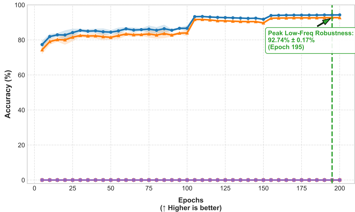
CIFAR-10 Test Accuracy vs. Epochs (5 Seeds Mean \pm SD)
