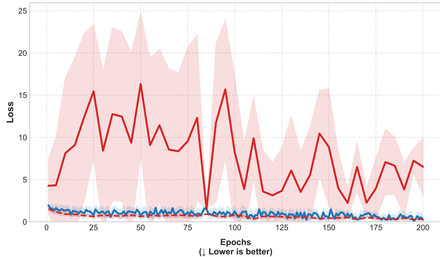
Training & Test Loss (5 Seeds Mean \pm SD)
