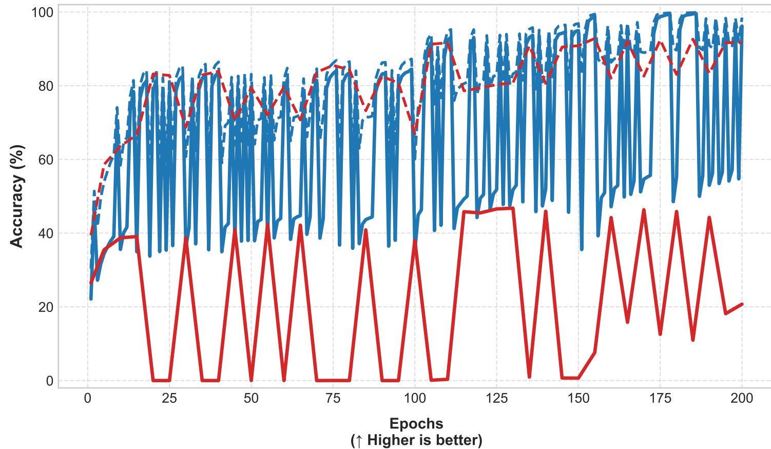
Training & Test Accuracy (TensorBoard Log)
