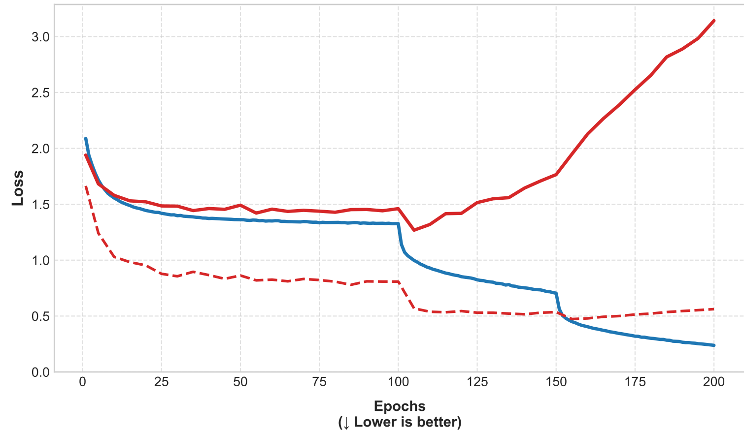
Training & Test Loss (TensorBoard Log)
