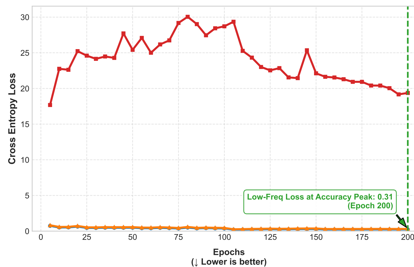
CIFAR-10 Test Loss vs. Epochs
