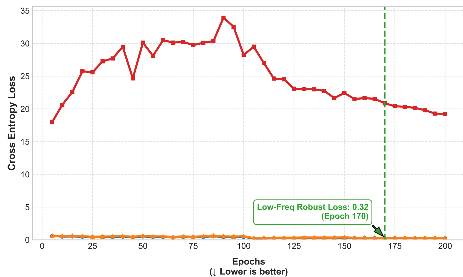
CIFAR-10 Test Loss vs. Epochs
