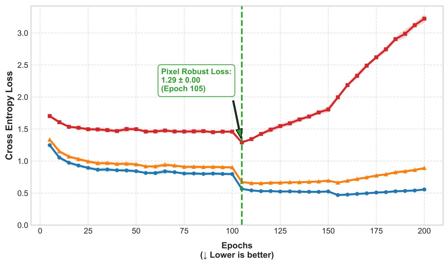
CIFAR-10 Test Loss vs. Epochs (5 Seeds Mean \pm SD)
