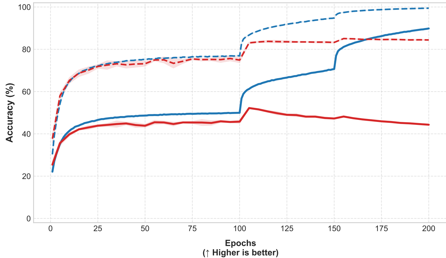
Training & Test Accuracy (5 Seeds Mean \pm SD)
