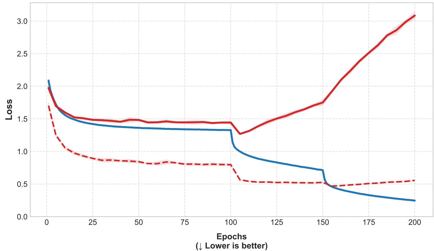
Training & Test Loss (5 Seeds Mean \pm SD)
