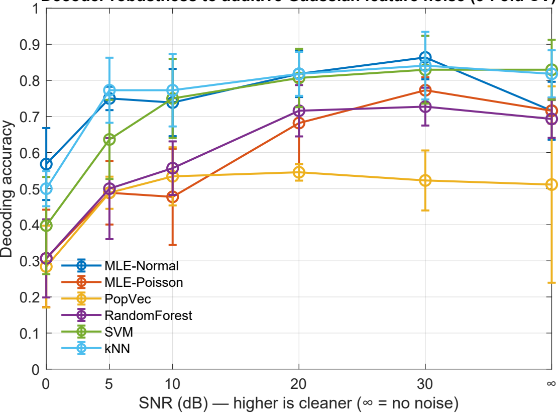
Decoder robustness to additive Gaussian feature noise (5-Fold CV)
