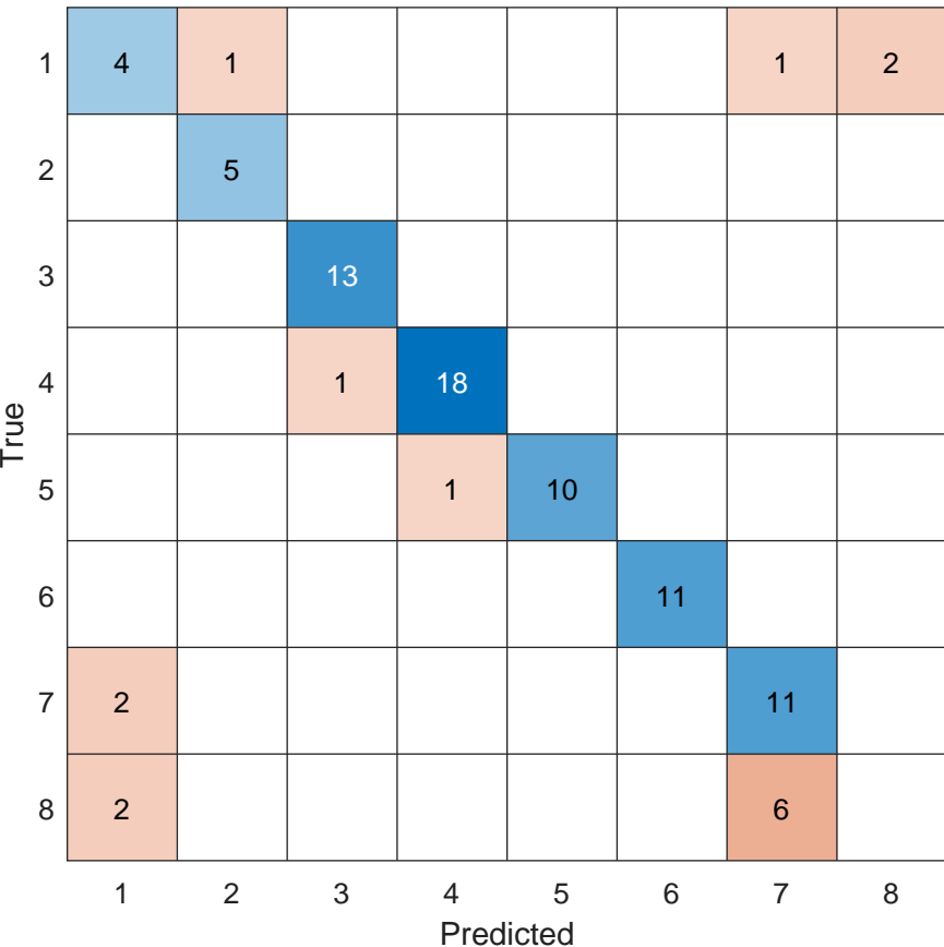
Confusion: kNN @ inf dB
