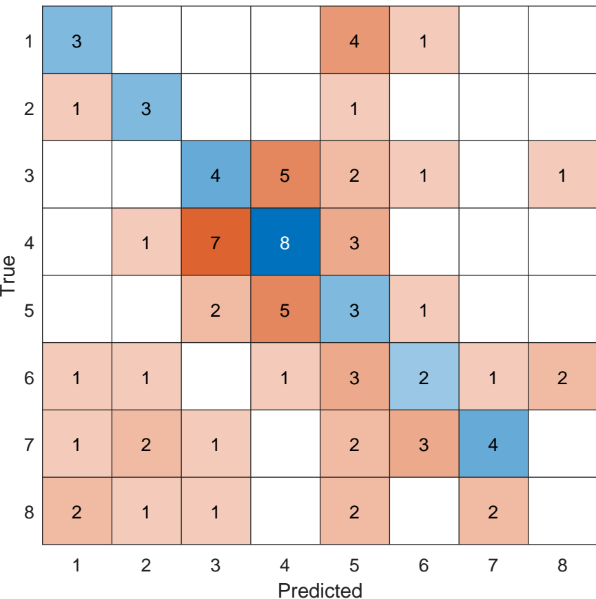
Confusion: MLE-Poisson @ 0 dB
