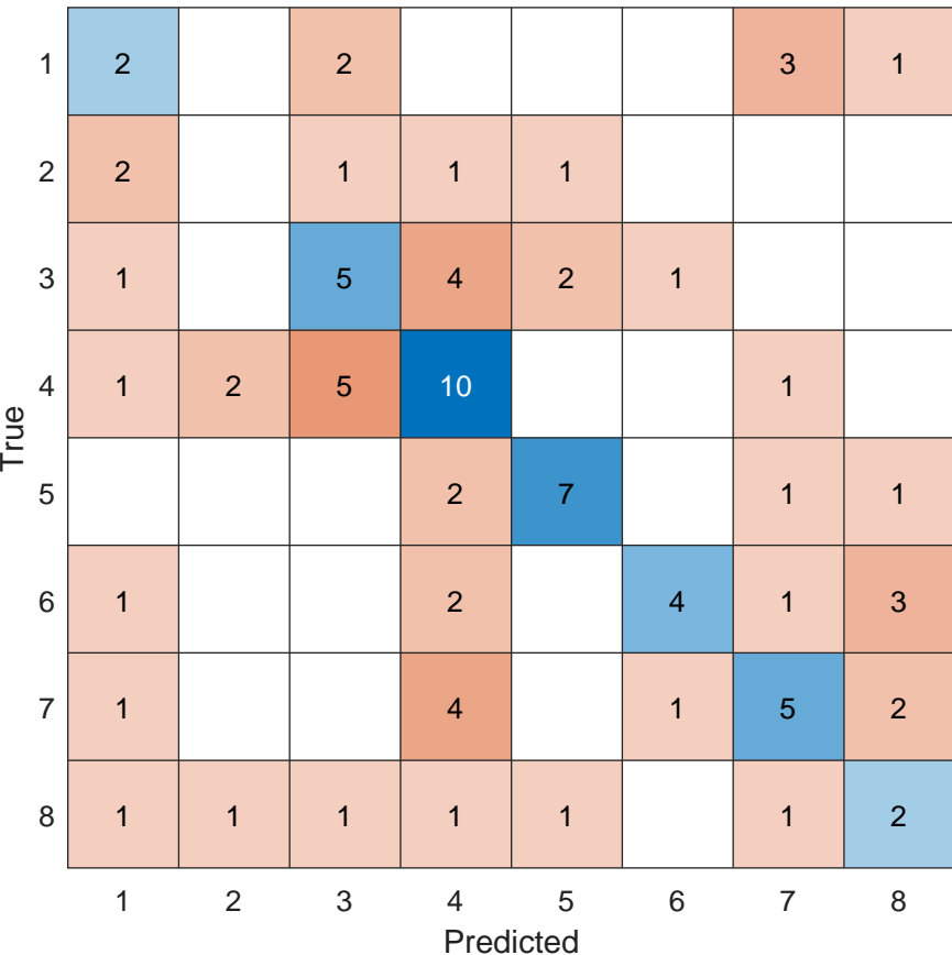
Confusion: SVM @ 0 dB
