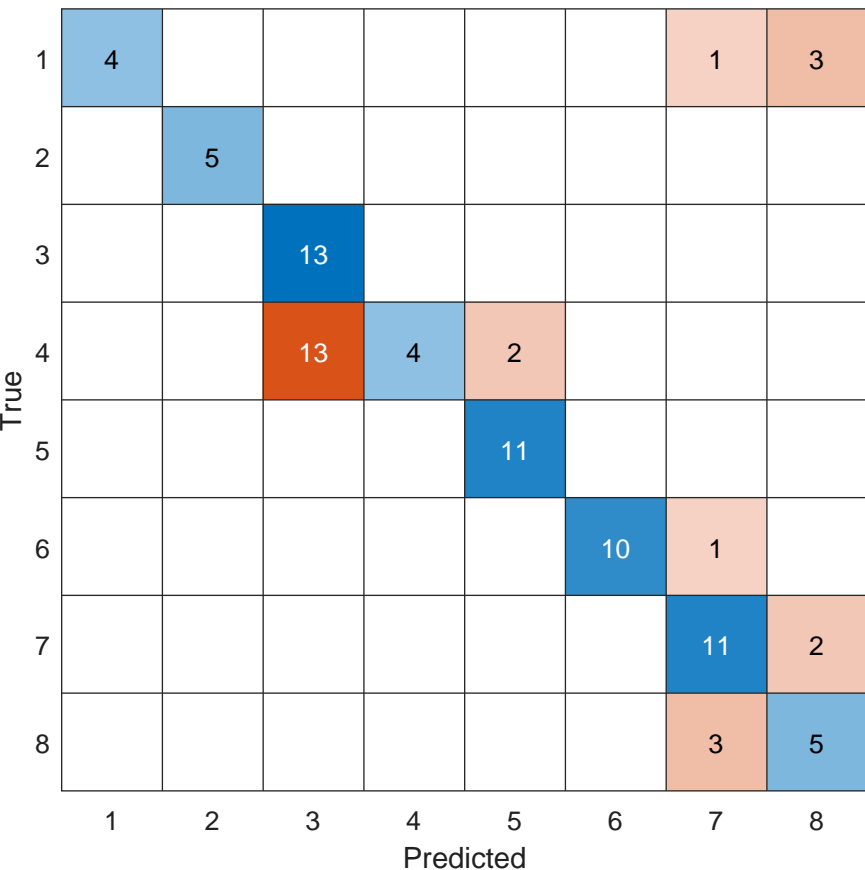
Confusion: MLE-Poisson @ inf dB
