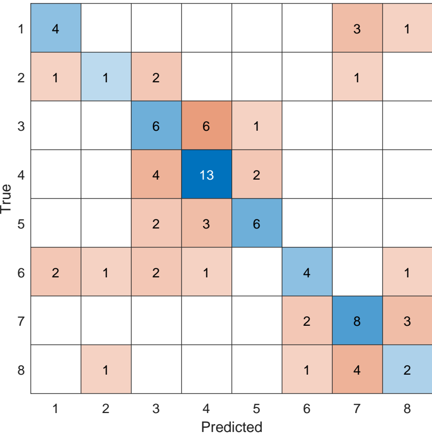
Confusion: kNN @ 0 dB
