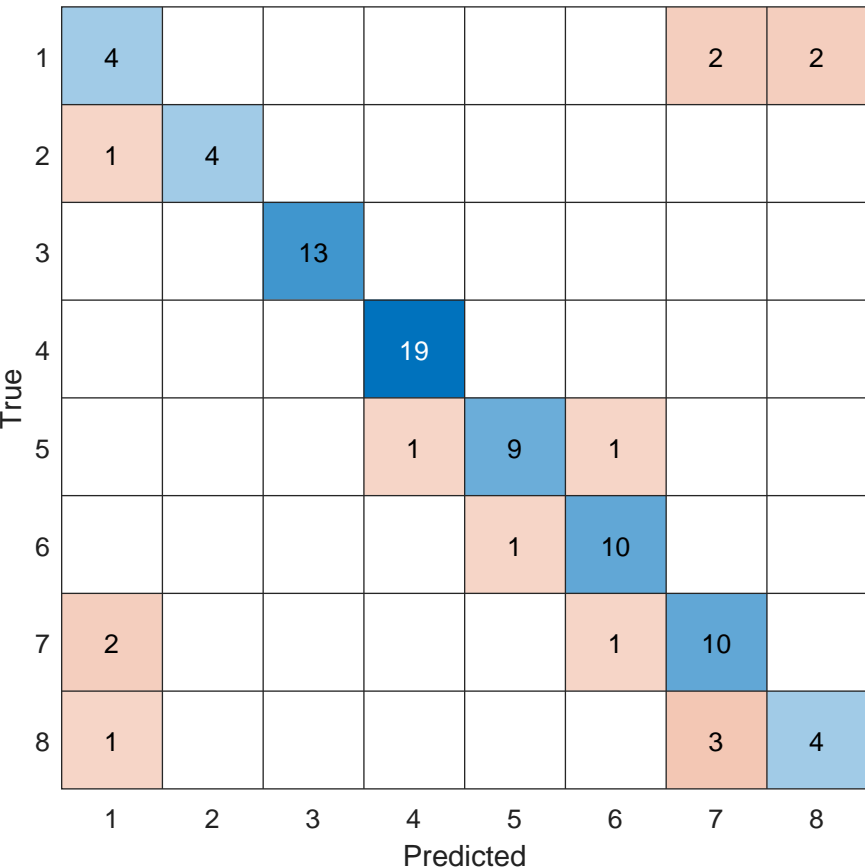
Confusion: SVM @ inf dB
