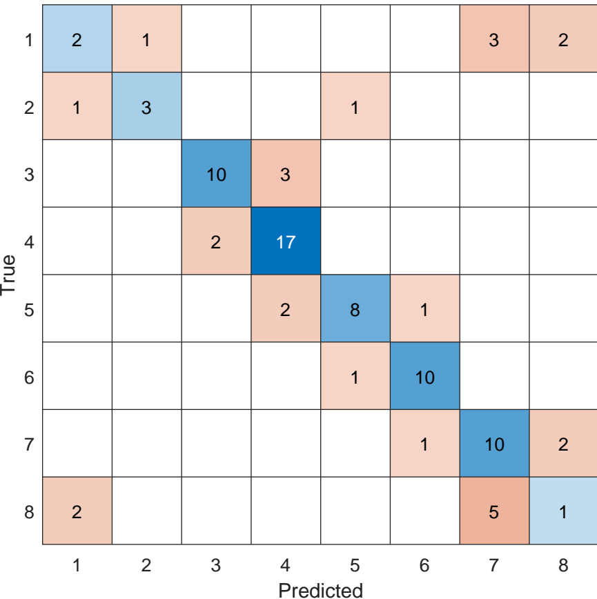
Confusion: RandomForest @ inf dB
