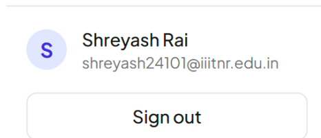
Figure 2.5: Logout Button
