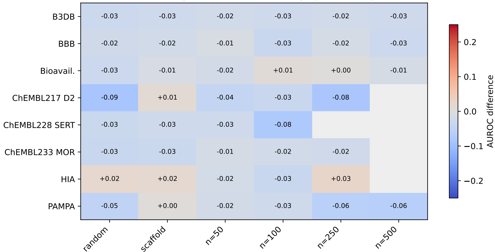
Best frozen embedding AUROC minus best fingerprint/descriptor baseline
