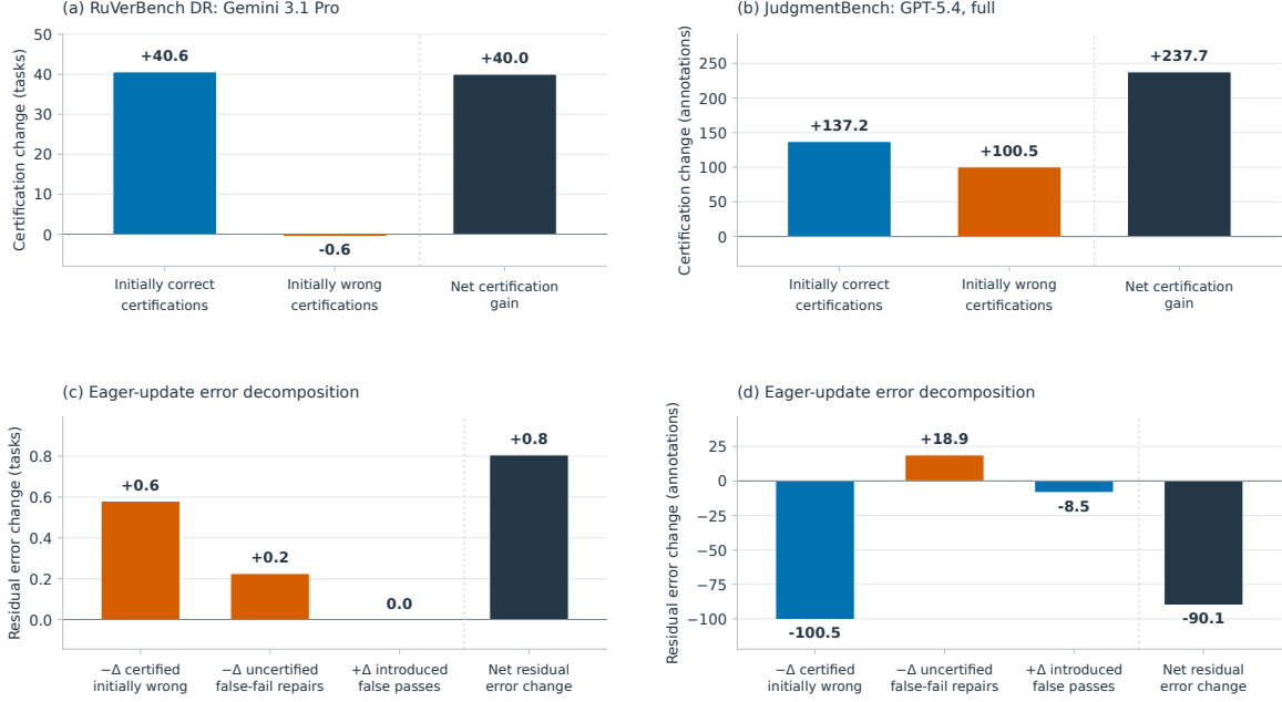
Figure 2: Allocation effects separated into where certificates are added and how residual disagreements change. Differences are fixed mix minus criterion SRS at a 20% budget, release task order, averaged across 31 paired orders at equal query counts. The columns show DR Gemini (284 tasks, 323 queries) and full JB GPT-5.4 (1,539 annotations, 4,697 queries). Components add before rounding. The DR error increase describes the original frame; its direction varies in the task-composition analysis.
