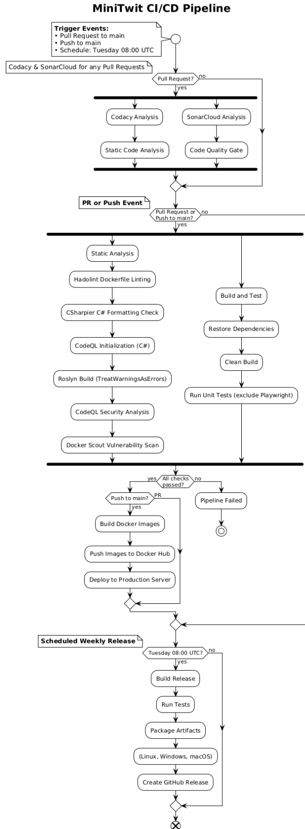
Figure 6: CI-CD pipeline
