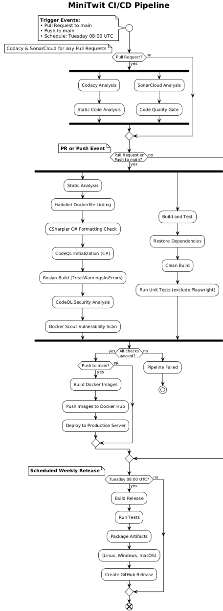
Figure 6: CI-CD pipeline
