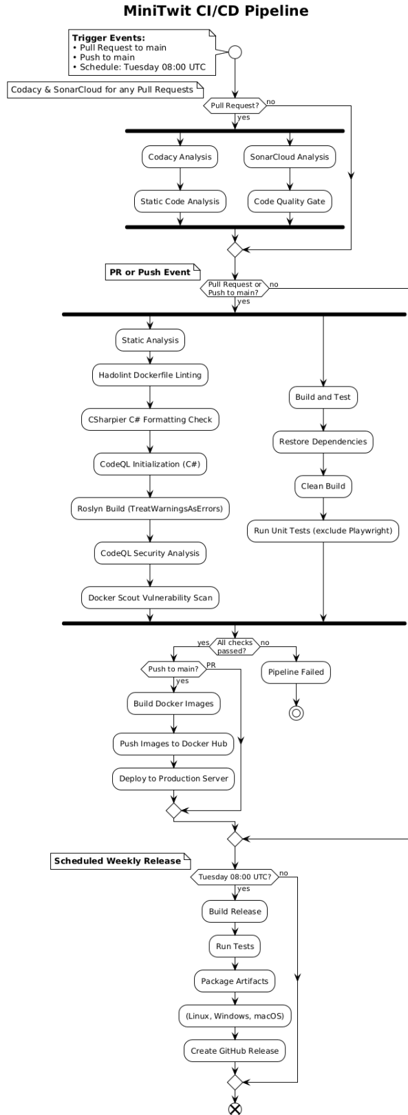
Figure 6: CI-CD pipeline
