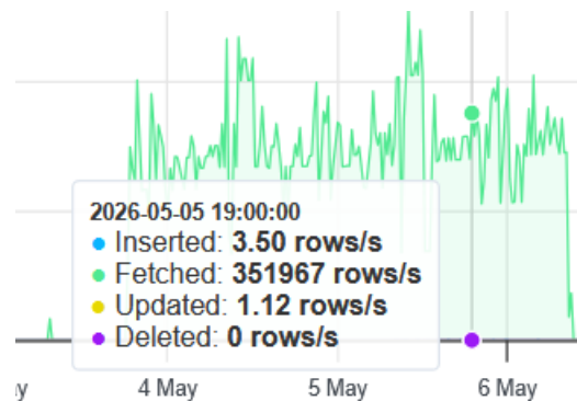
Figure 2: Database load
