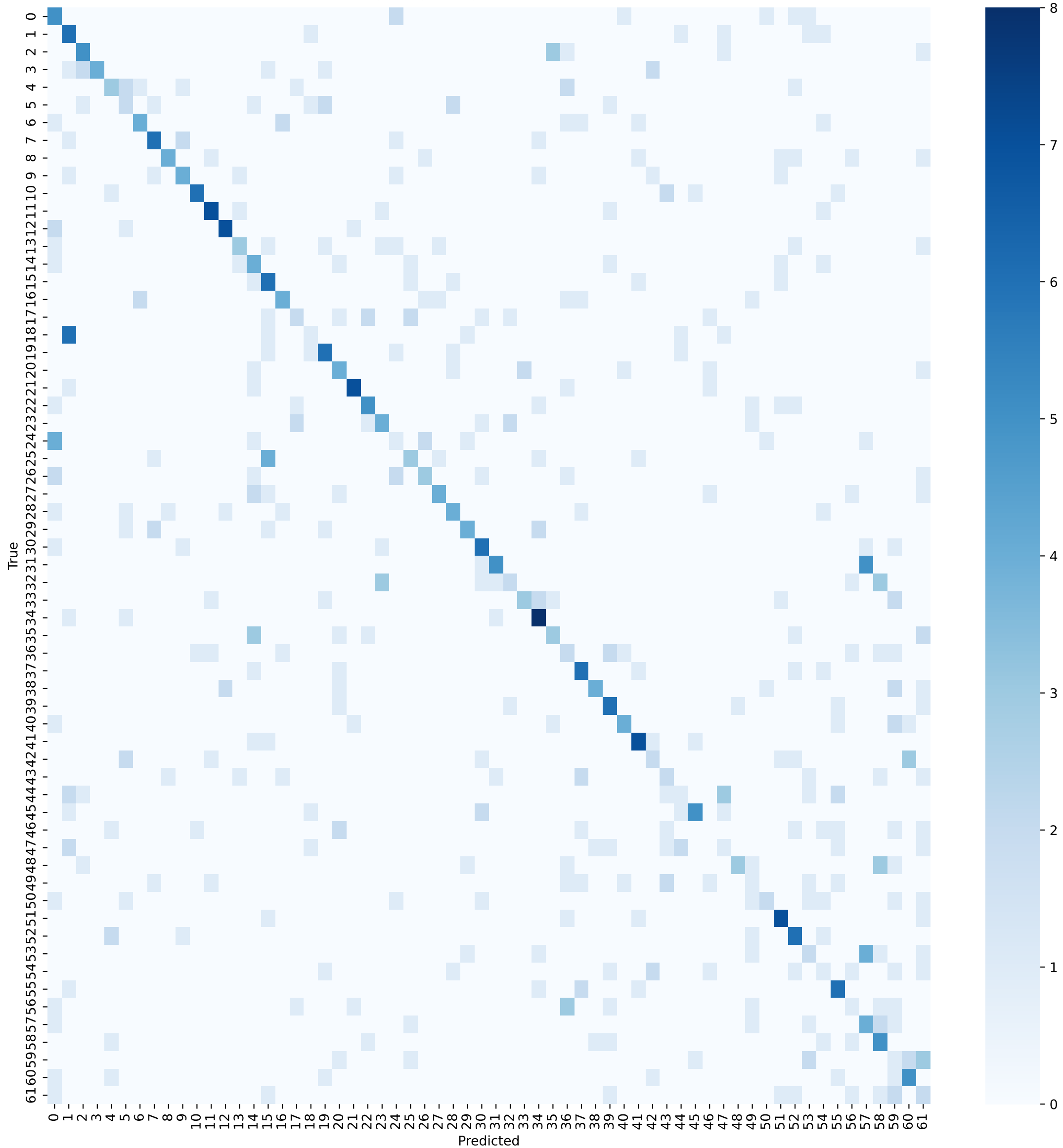
Confusion Matrix - Tuned MLP
