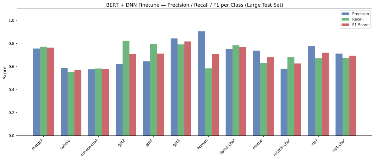
Figure 5.3: BERT + DNN Finetune — Precision, recall, and F1 score per class on the large test set.
