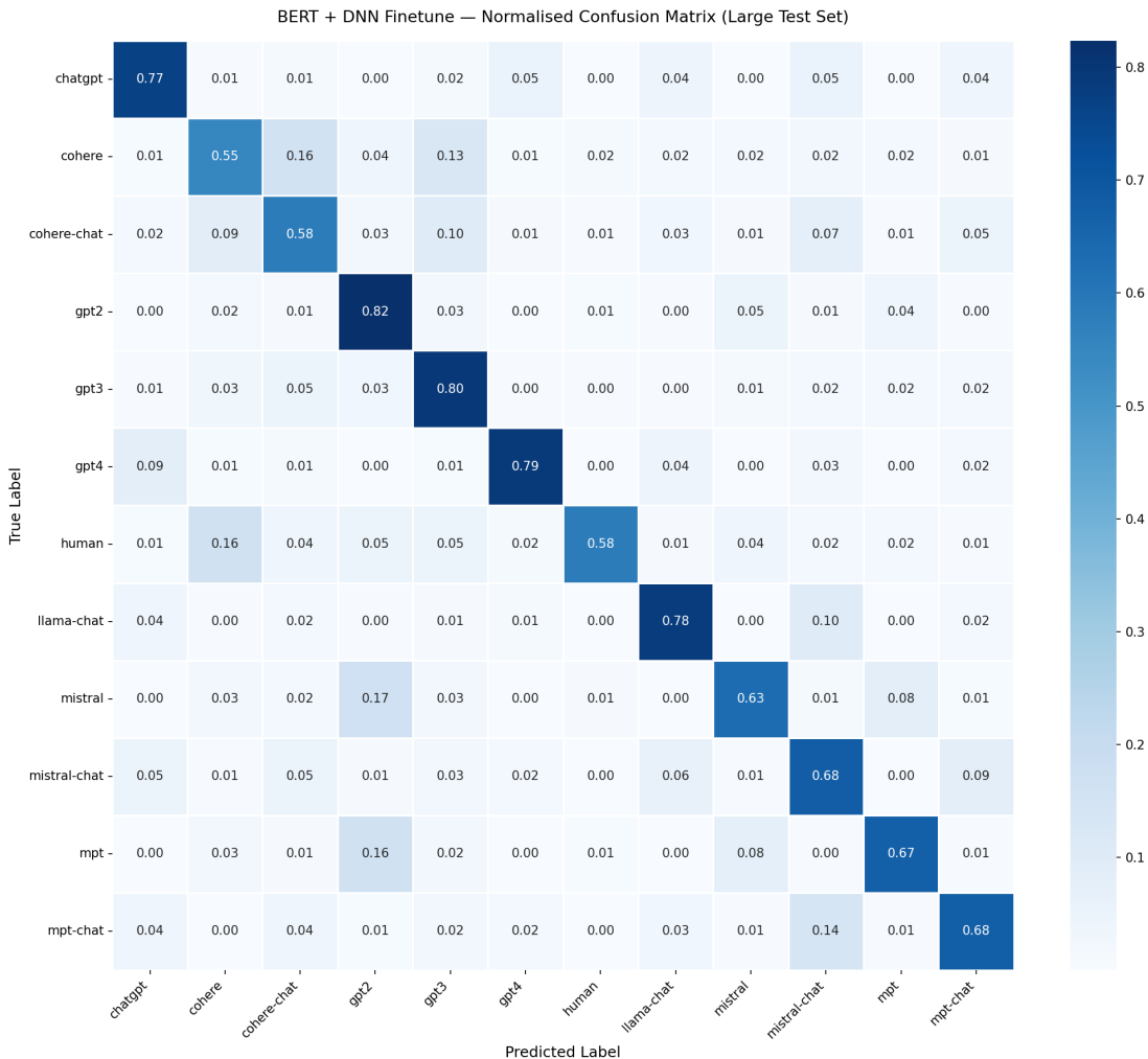
Figure 5.1: BERT + DNN Finetune — Row-normalised confusion matrix on the large test set. Diagonal values represent per-class recall.
