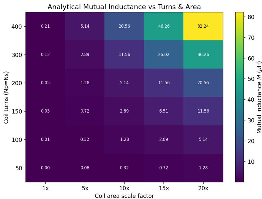
Figure 8 — Analytical mutual inductance vs turns and coil-area scale ( \mu\text{H} ). Annotated cells make the N^2 \times \text{area} scaling directly readable.
