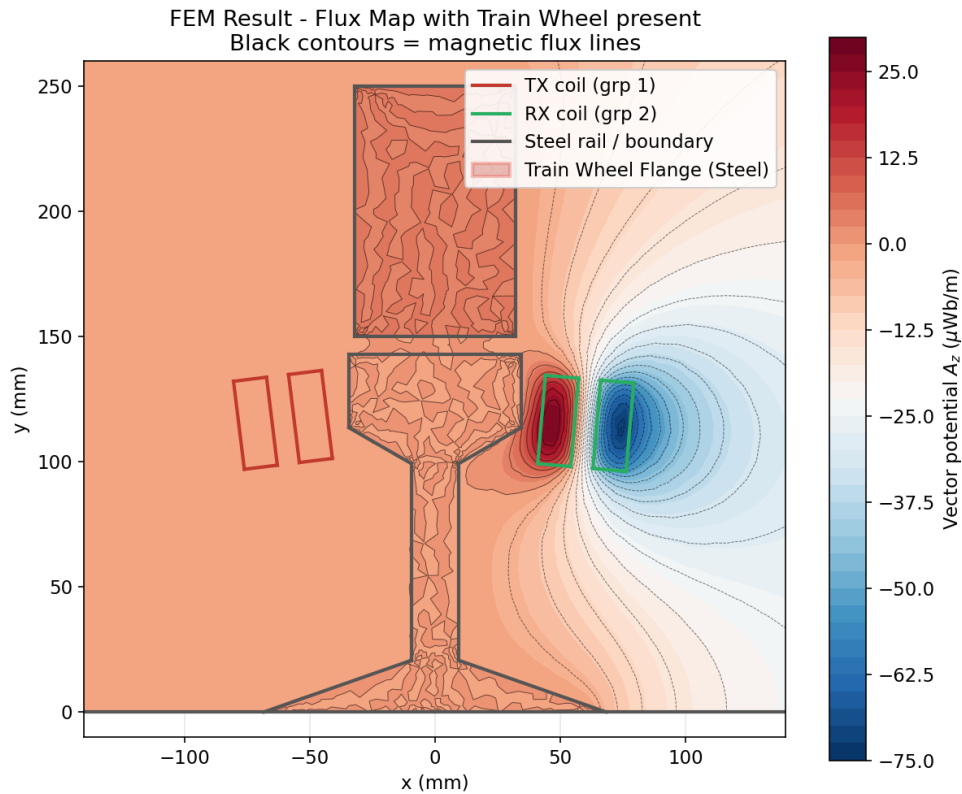
Figure 4 — The solved field with the steel wheel in the coil-to-coil flux path; the shaded red rectangle marks the wheel flange (rendered by the new generate_wheel_figure.py from the wheel experiment's own solution). Compare with Figure 2: the flux that previously arced across to the RX coil now terminates on and swirls inside the wheel.
