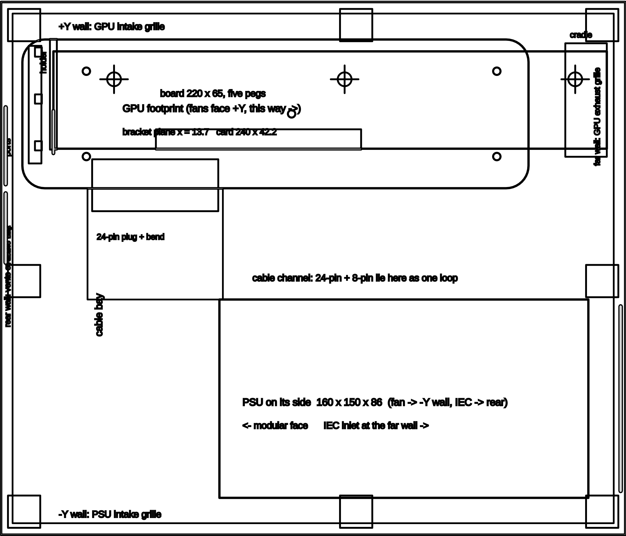
xgm-lite-frame floor plan 1:1 outside 270.7 x 231 mm (board origin = its rear/24-pin corner)
